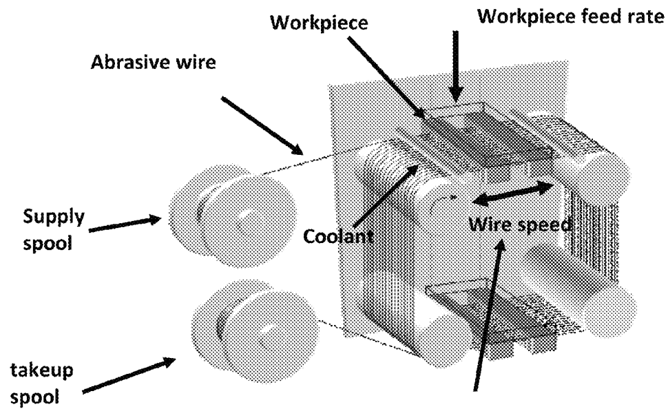
Reel to Reel Machine Set Up
