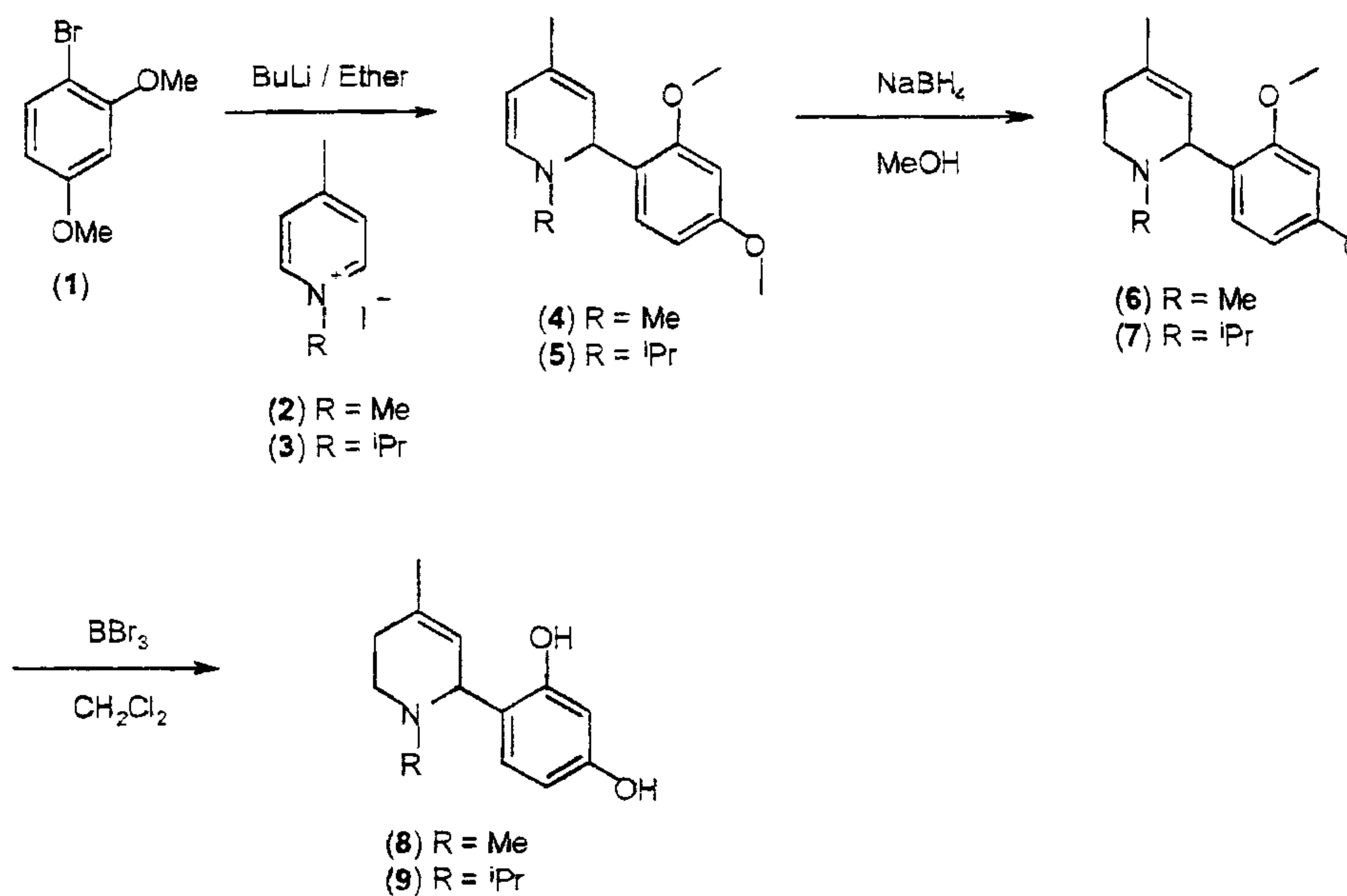
Scheme 1
