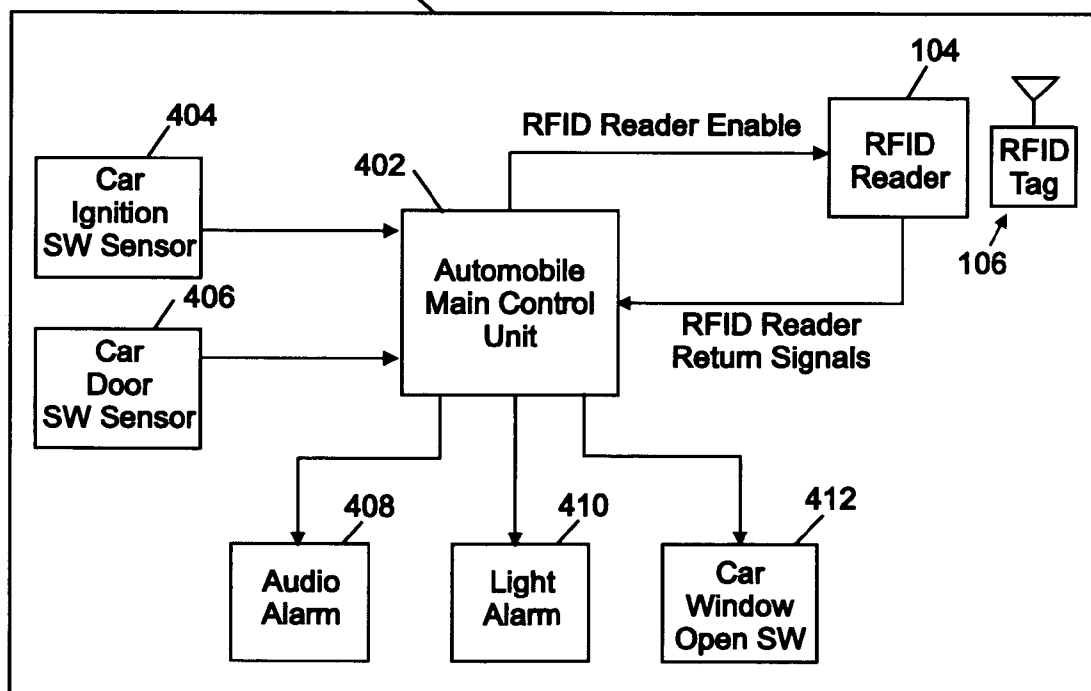
Overall RFID Child Safety System 400
