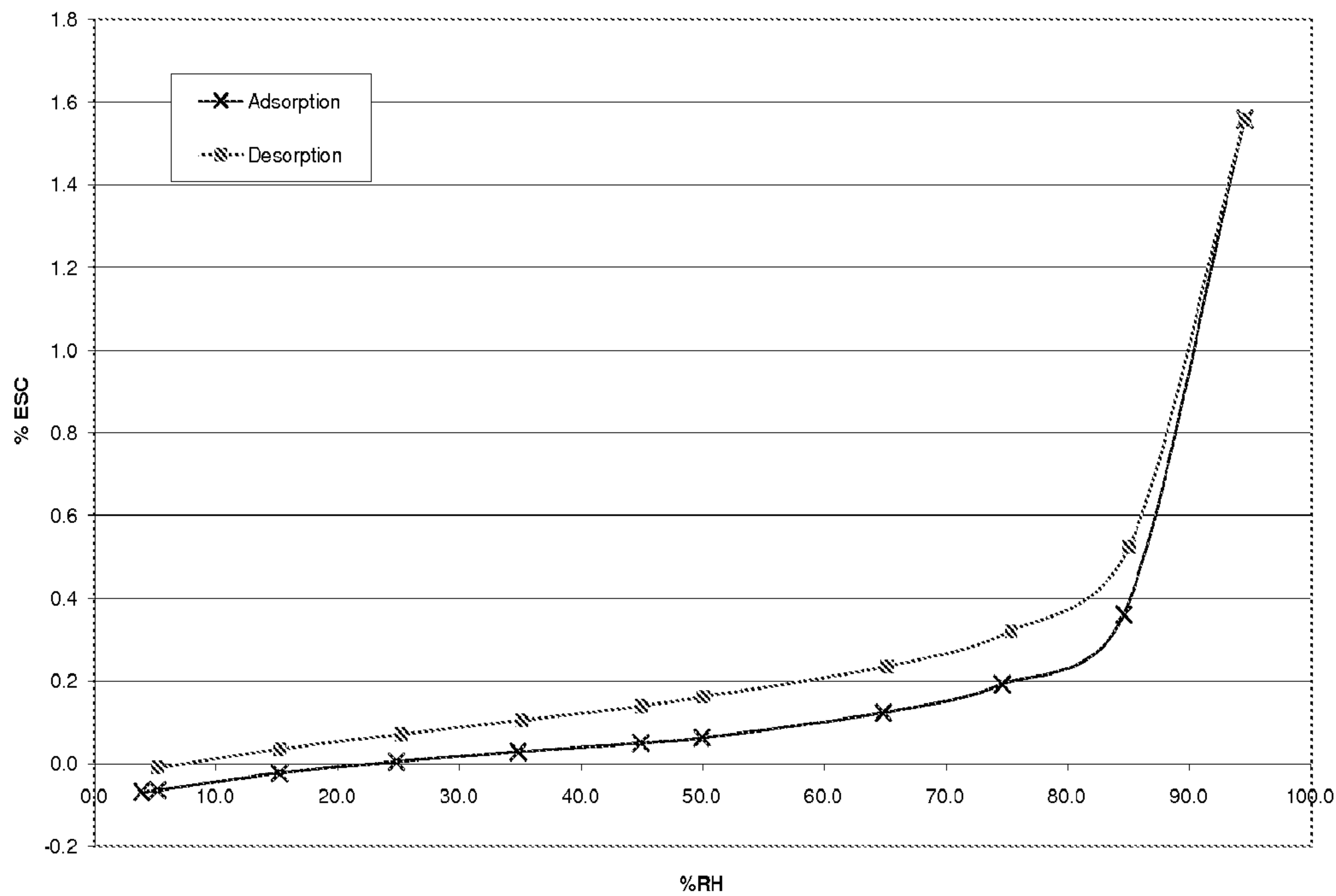
Moisture Sorption of Compound (I), Form N-1
