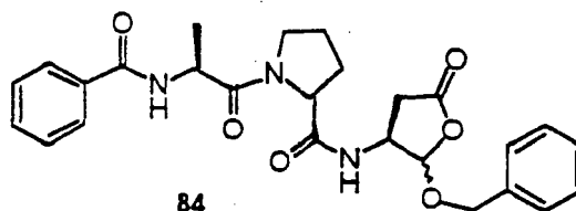
1-(2-Benzoylamino-propionyl)-pyrrolidine-2-carboxylic acid (2-benzyloxy-5-oxo-tetrahydro-furan-3-yl)-amide (84).
