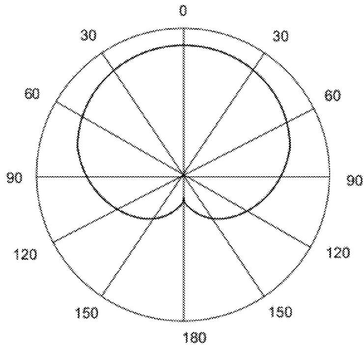
FIG. 2 (PRIOR ART)
