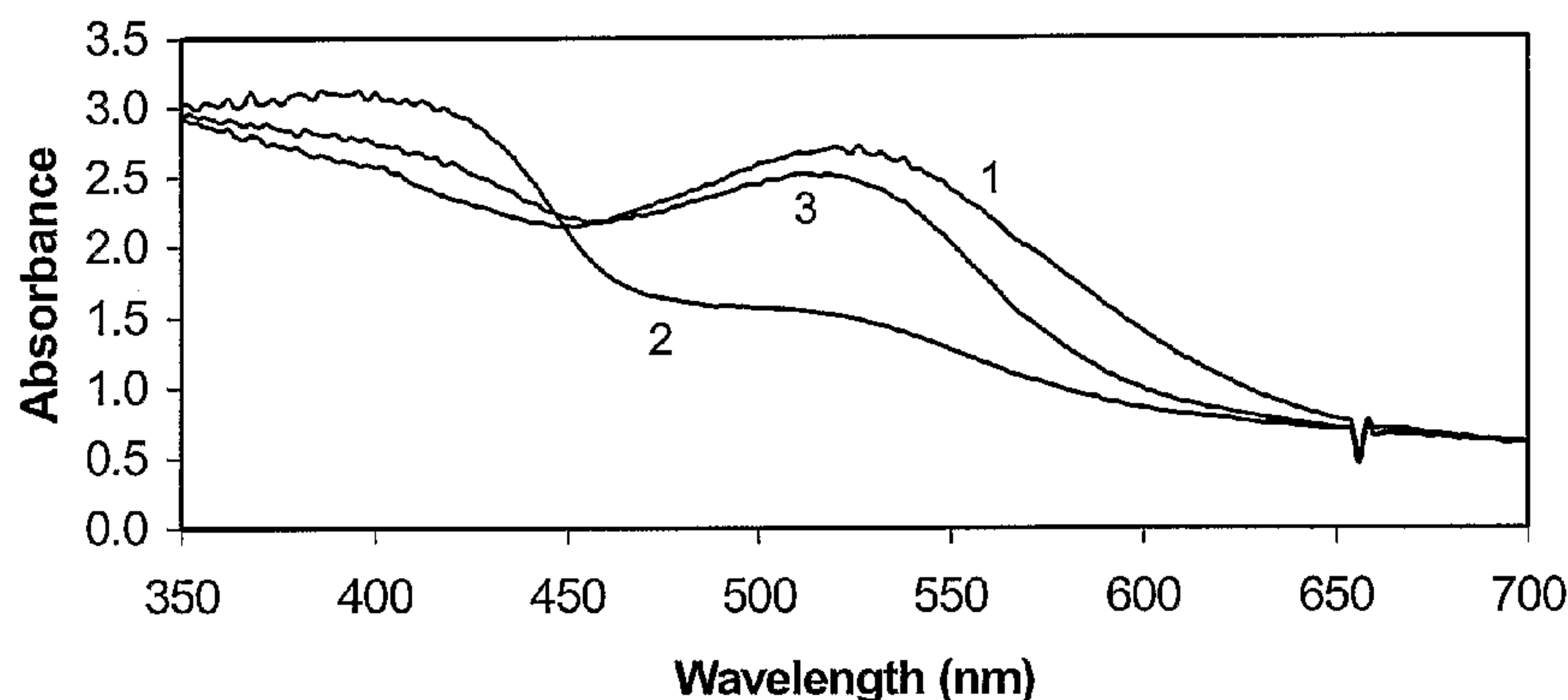
BR/PR Data Storage Spectra (set1)
