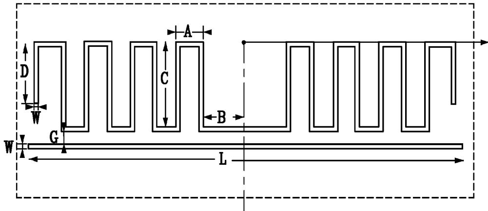
Meandering dipole antenna diagram
