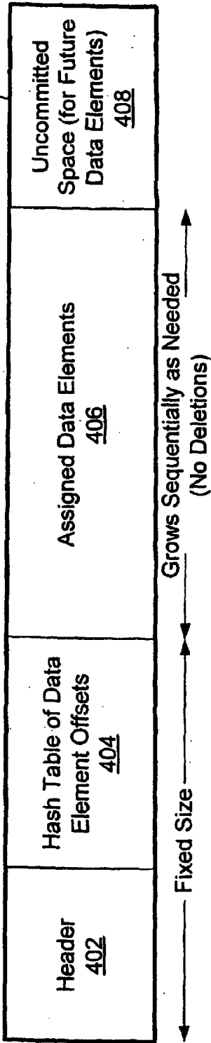
FIG. 4a: Central Cache File Structure
