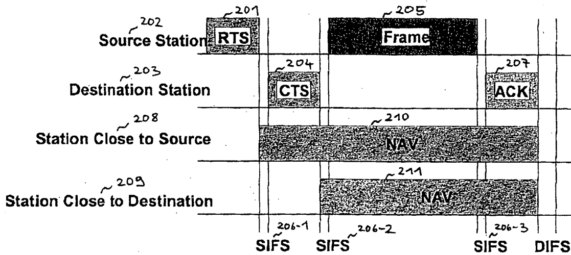
Fig. 2 (prior art)
