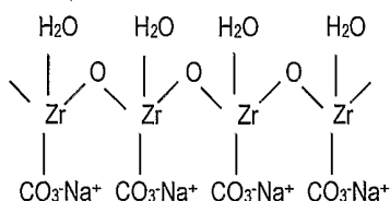
Molecular Structure of SZC before Titration
