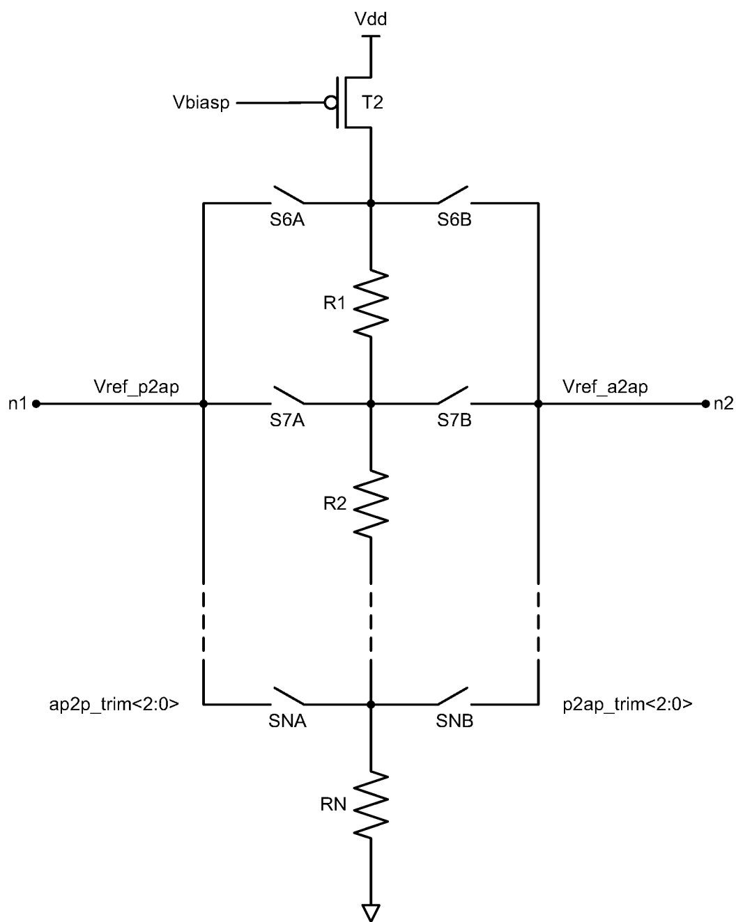
Reference Voltage Generator 104
