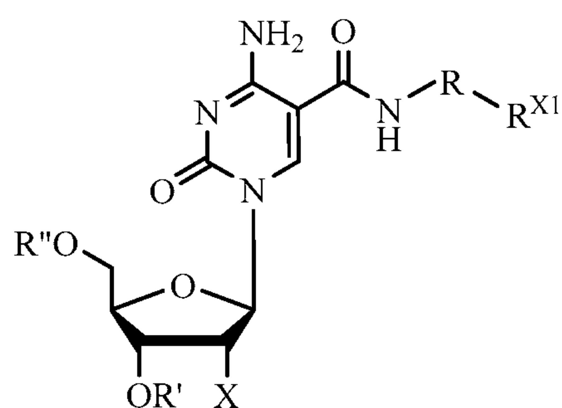
Formula I
