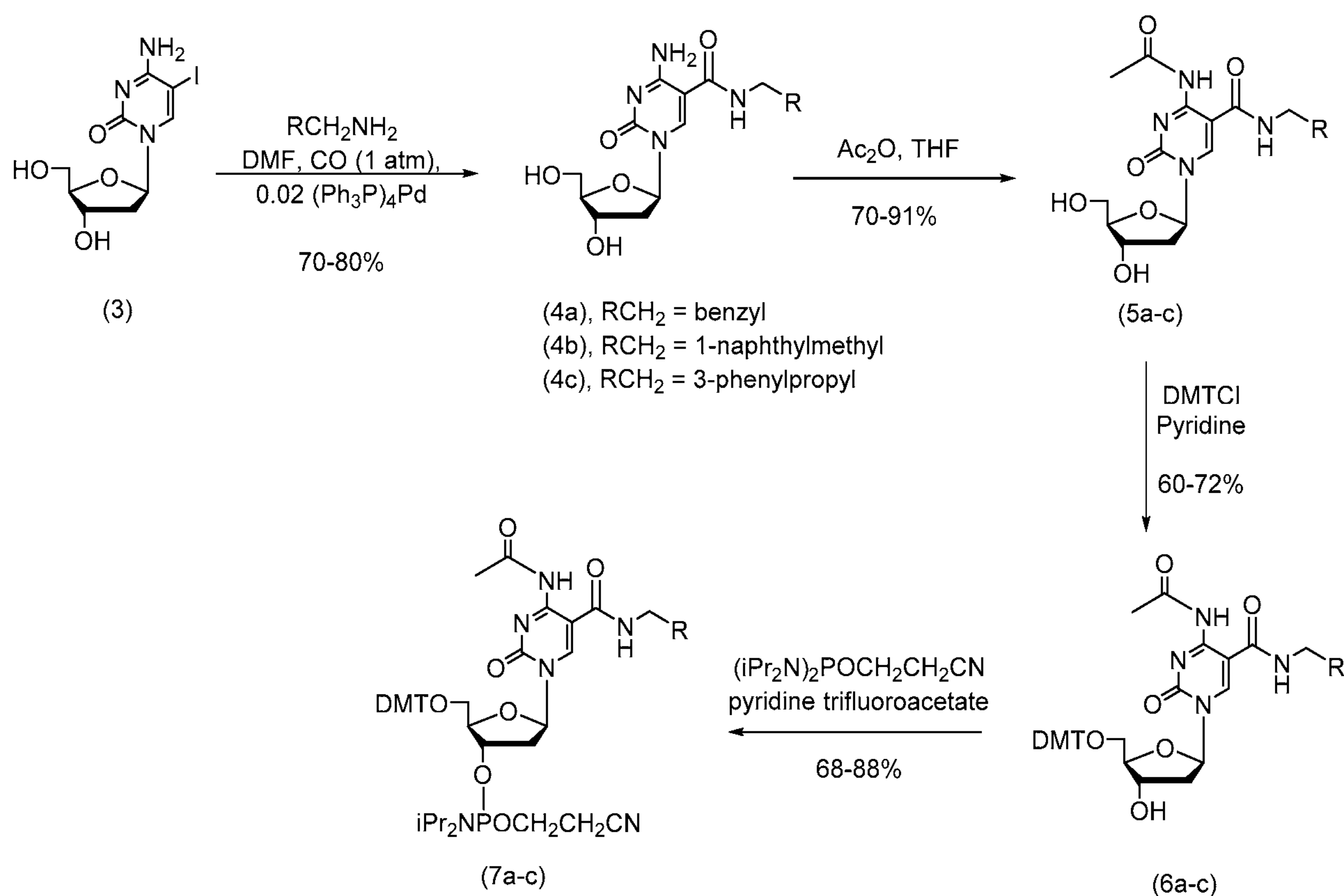
Scheme 1
