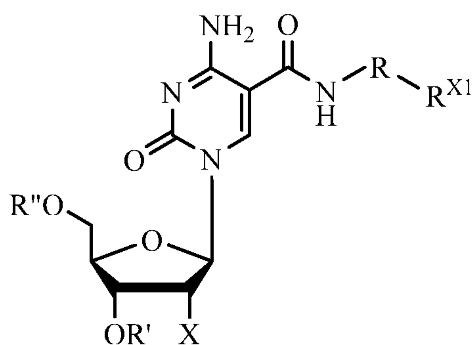
Formula I
