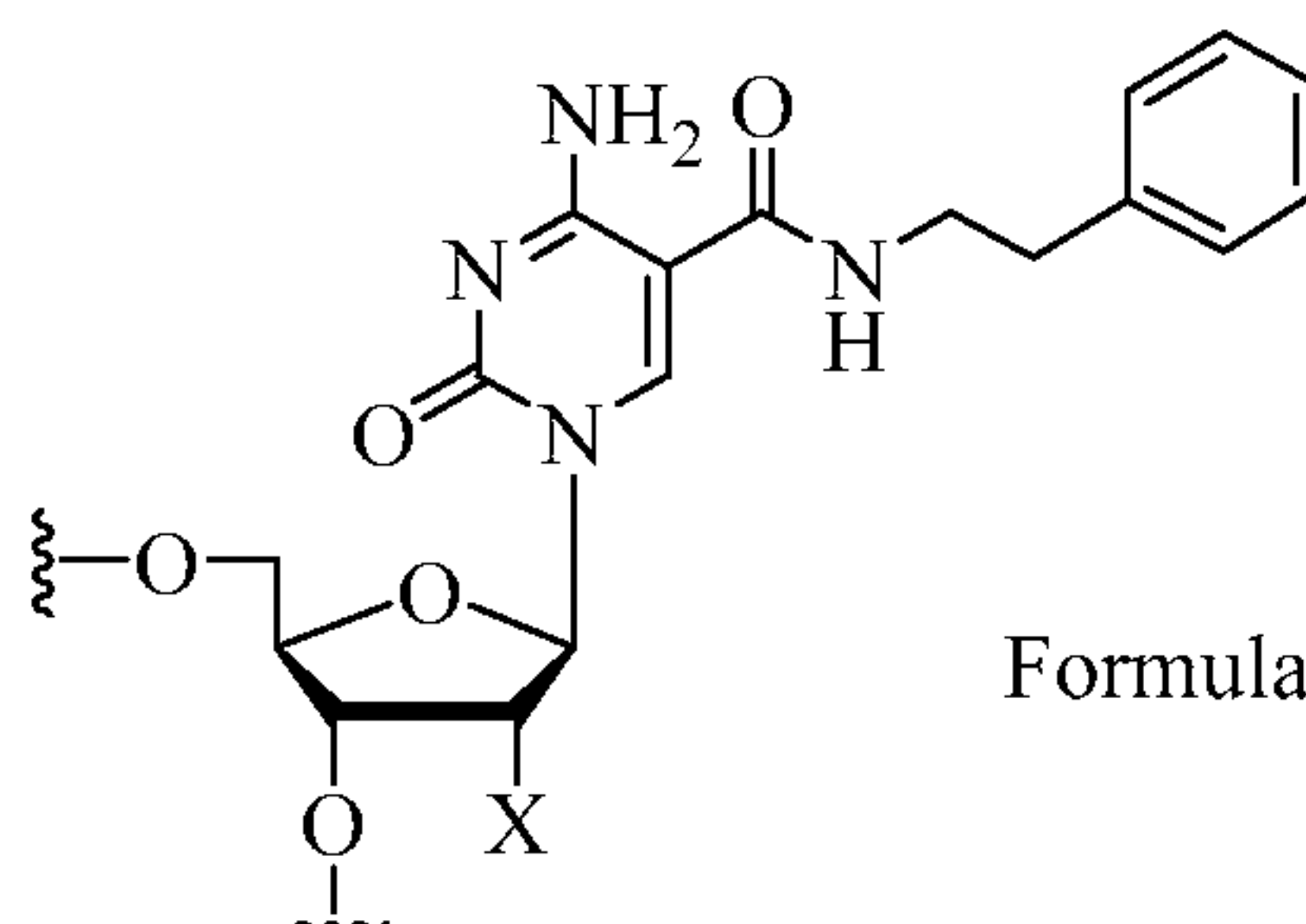
Formula IIA;
