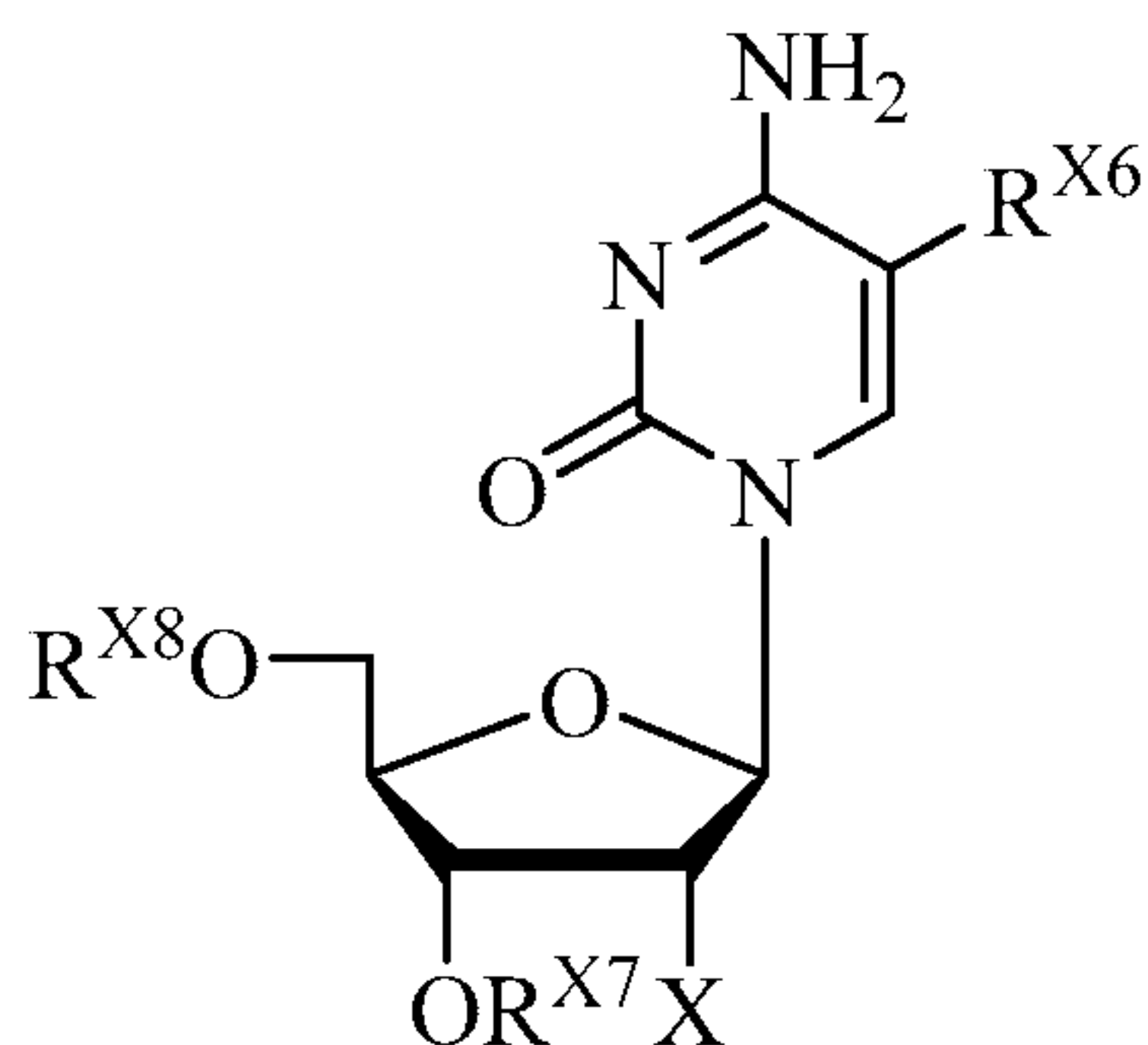
Formula IX
