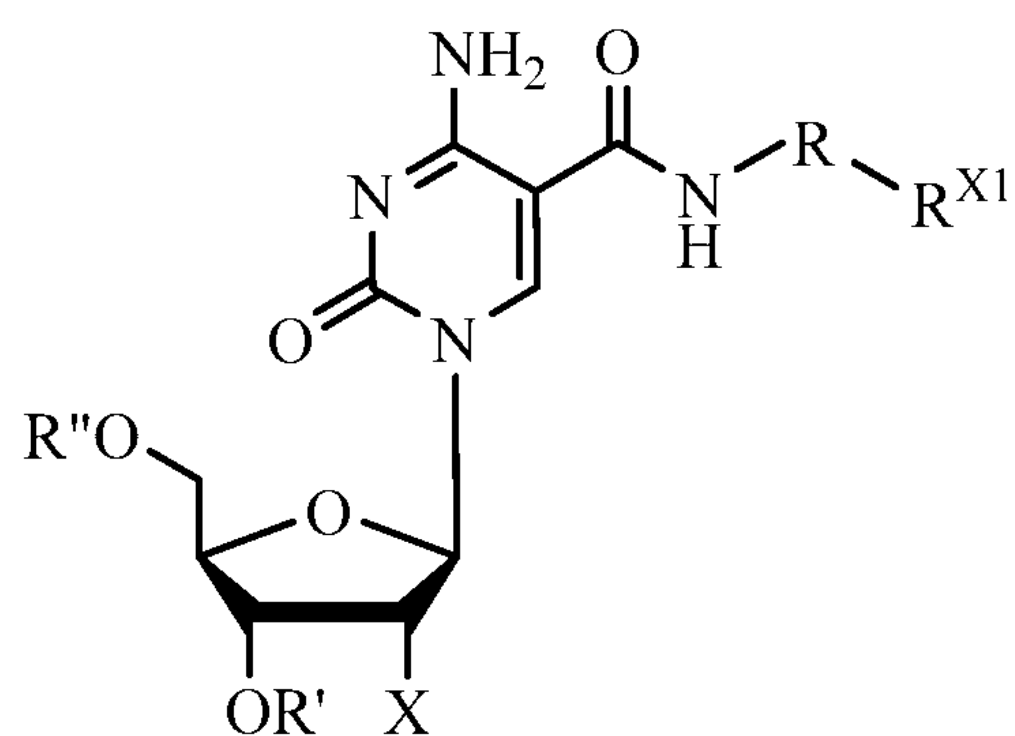
Formula I
