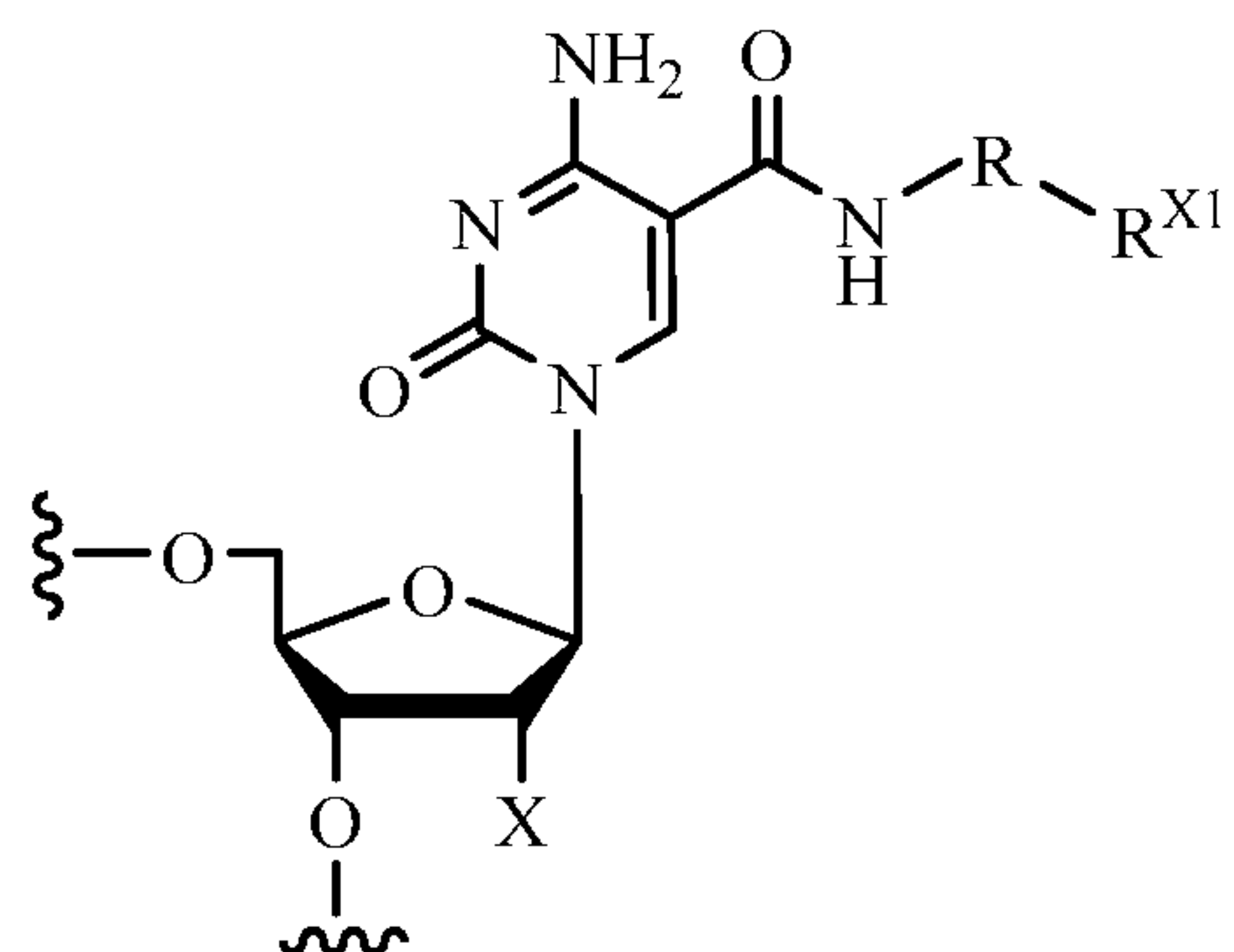
Formula IA
