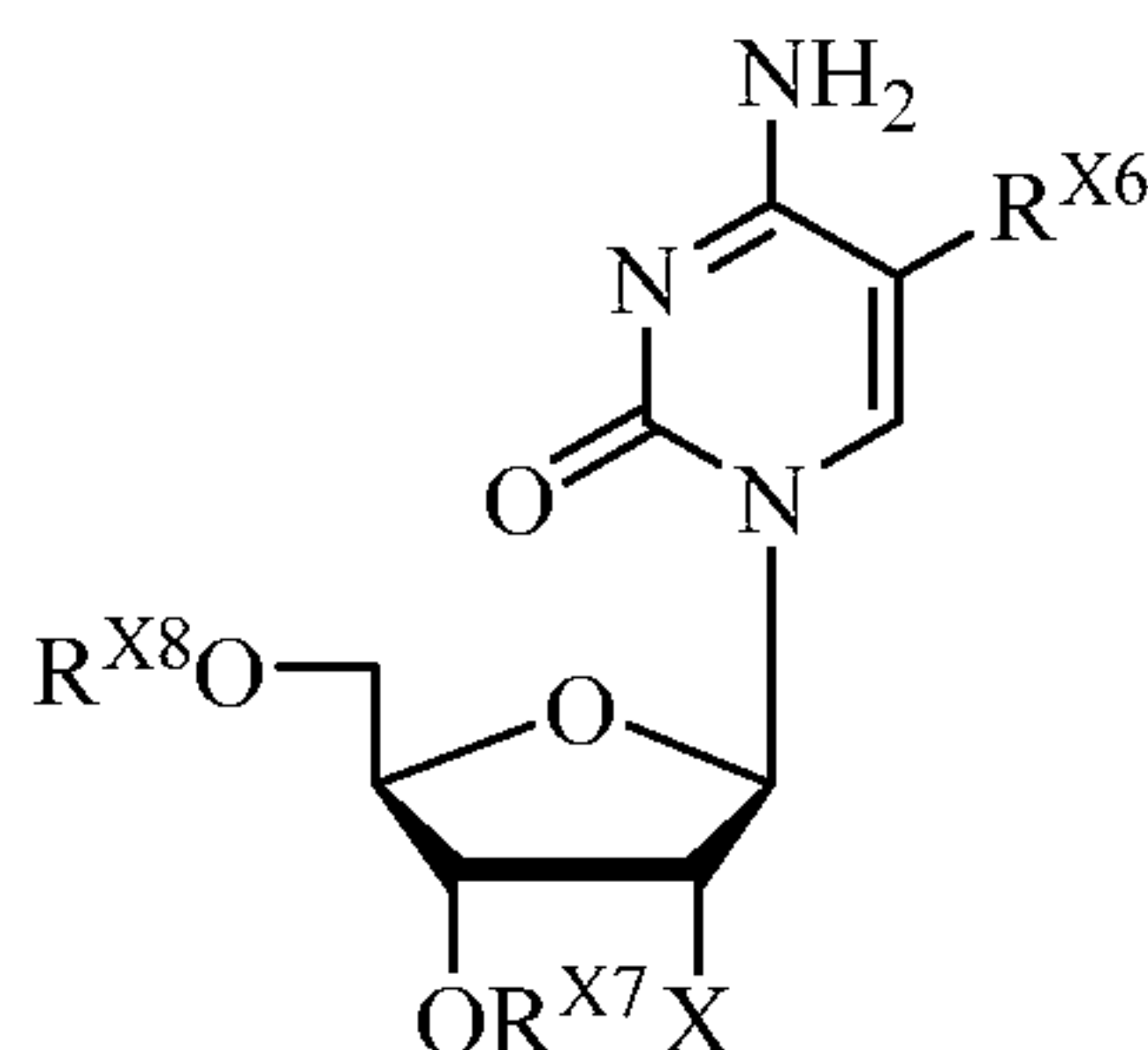
Formula IX
