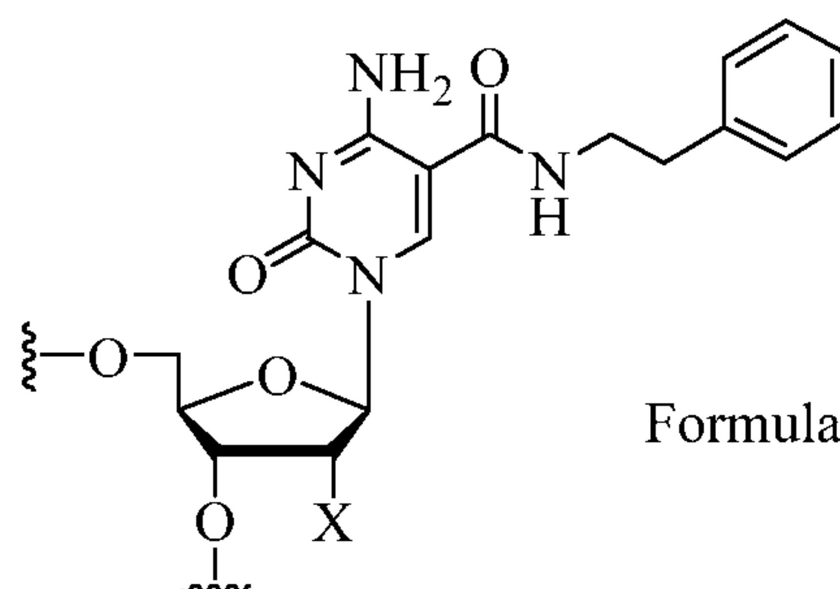
Formula IIA;
