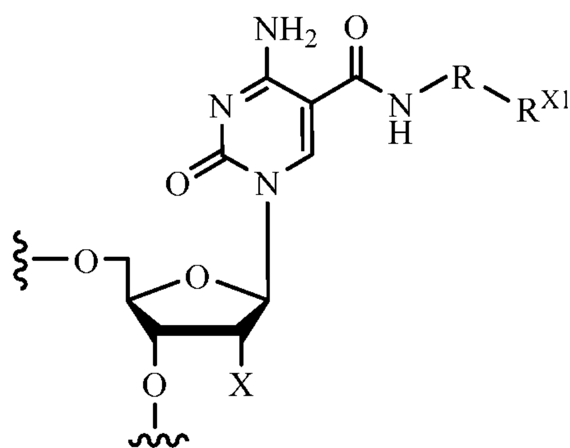
Formula IA
