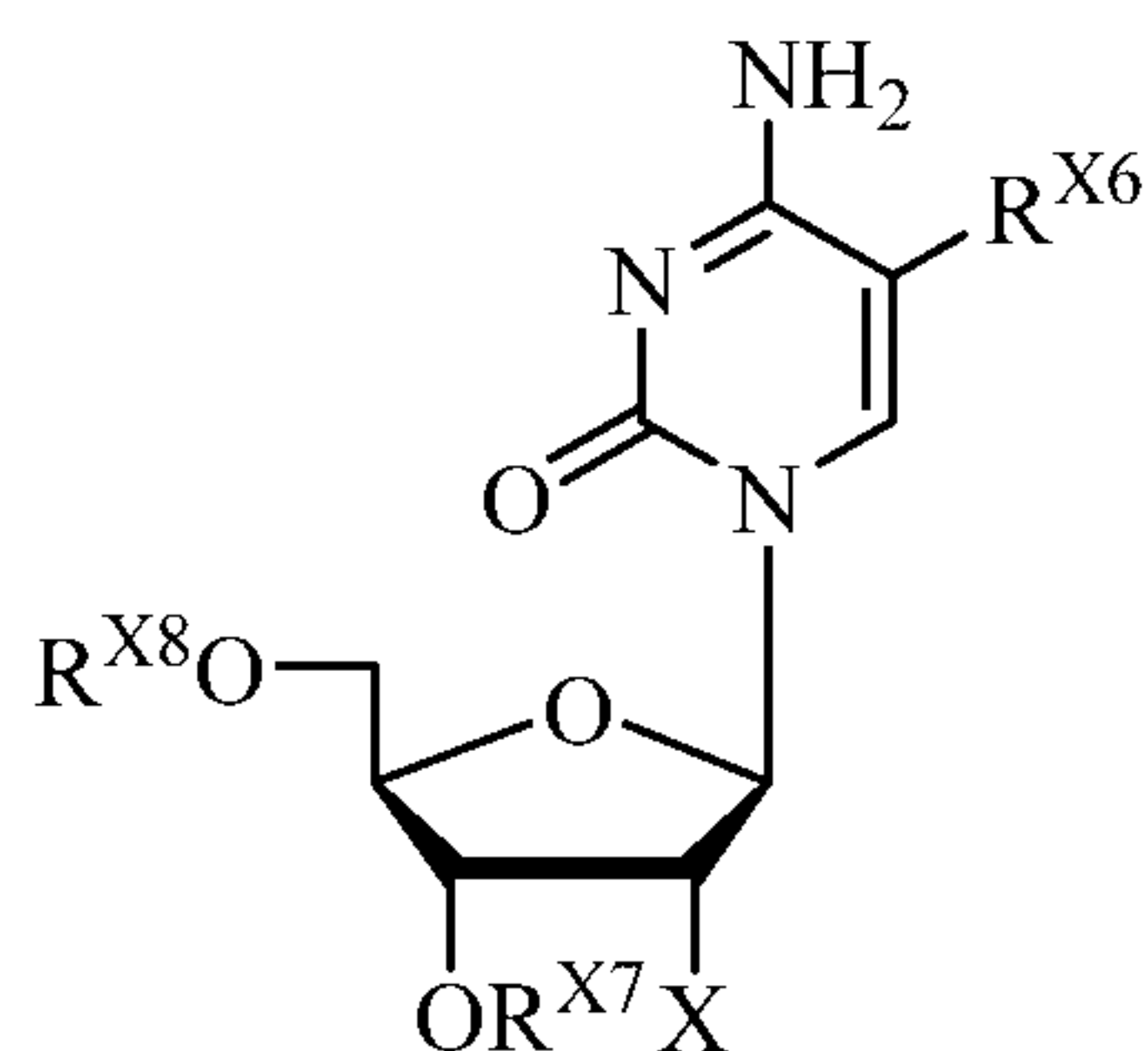
Formula IX
