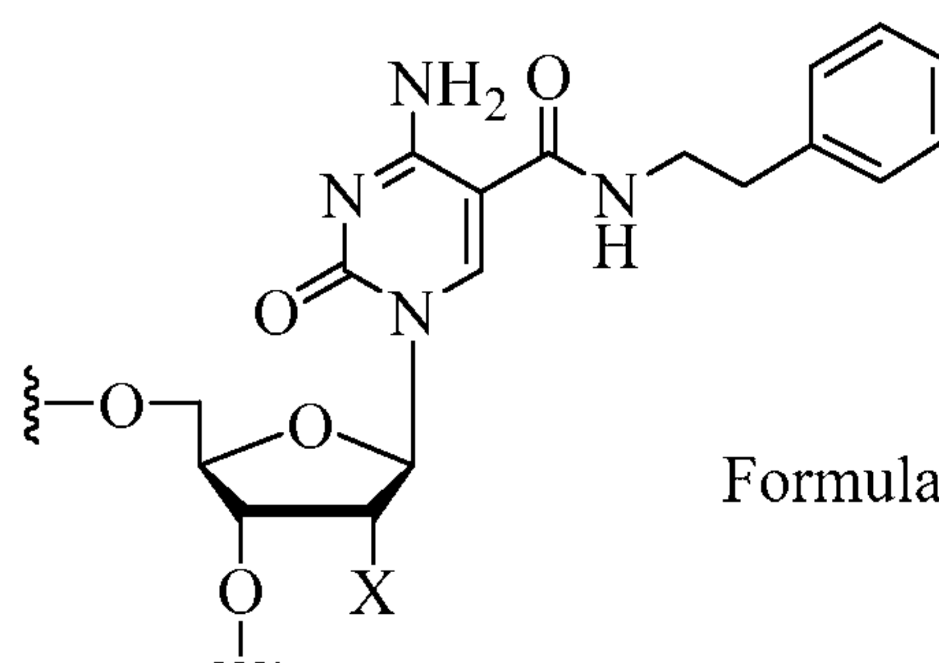
Formula IIA;
