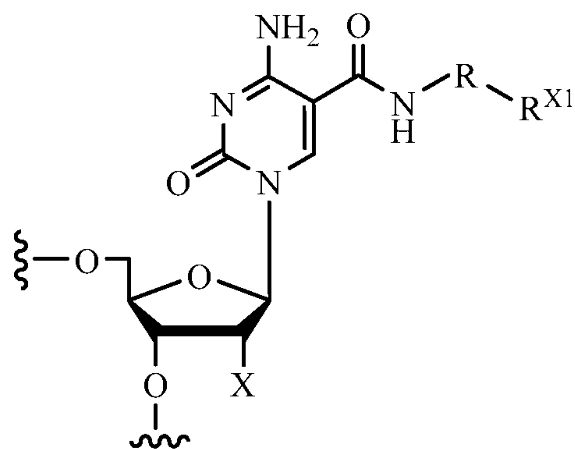
Formula IA
