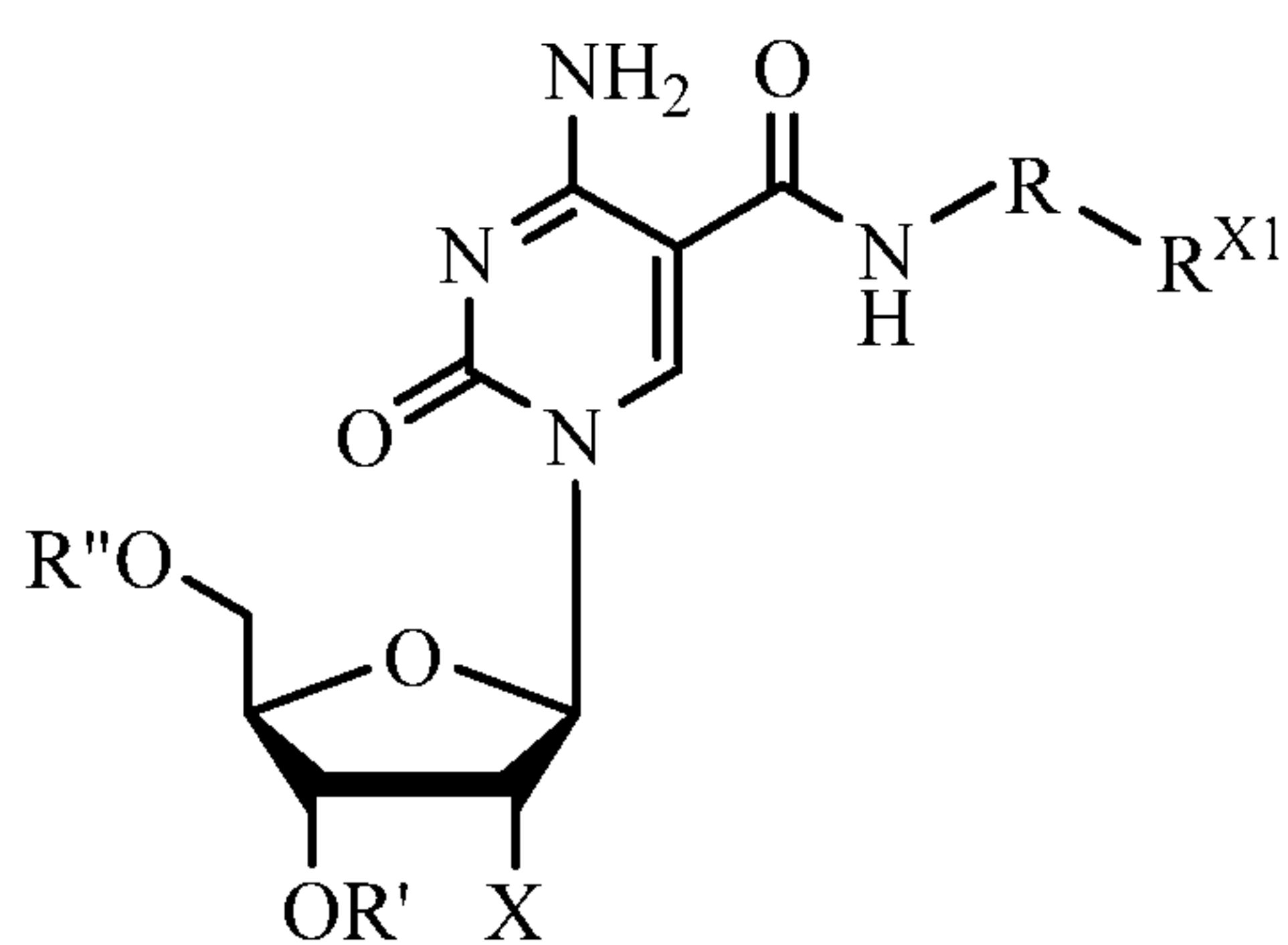
Formula I
