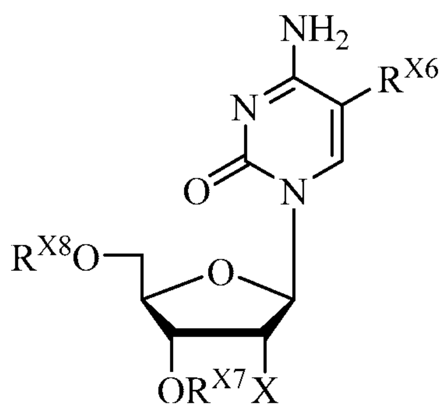
Formula IX
