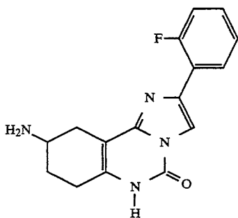
Compound 29 40
