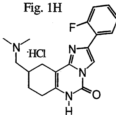
Compound 24
