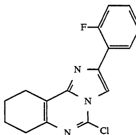
Compound 28 5
