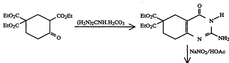
Scheme I
