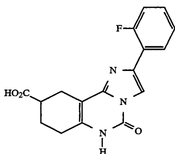
Compound 17
