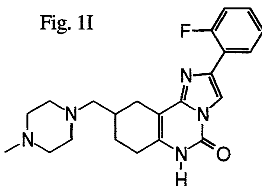
Compound 25
