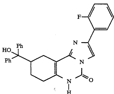
Compound 46
