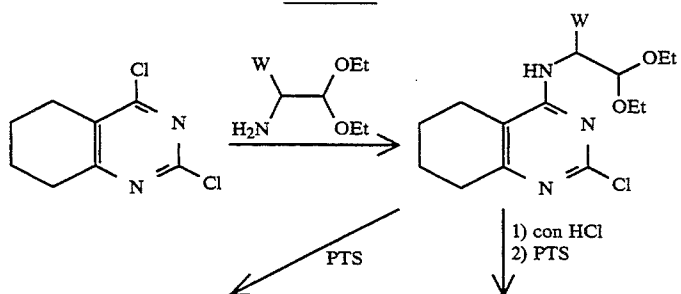
Scheme II
