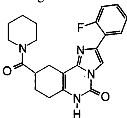
Compound 21
