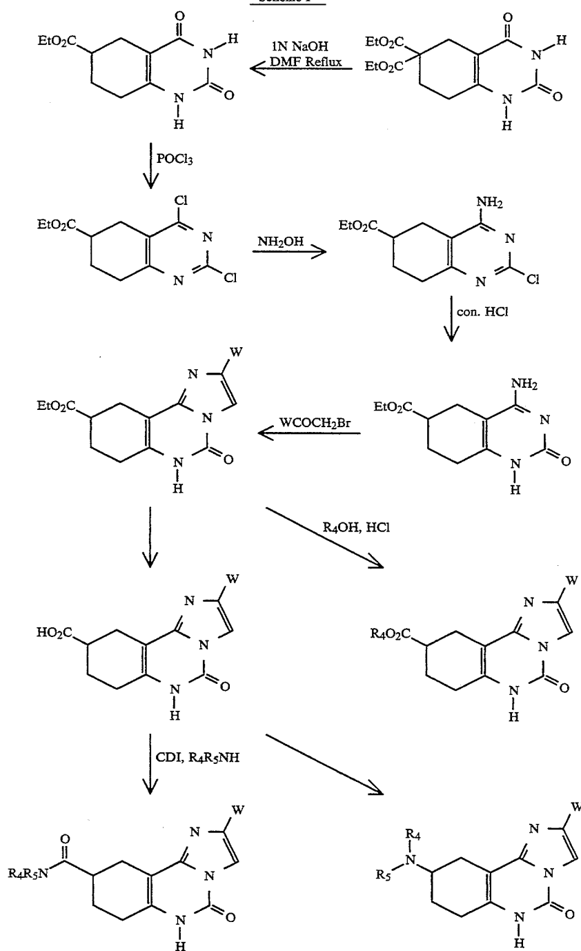
Scheme I
