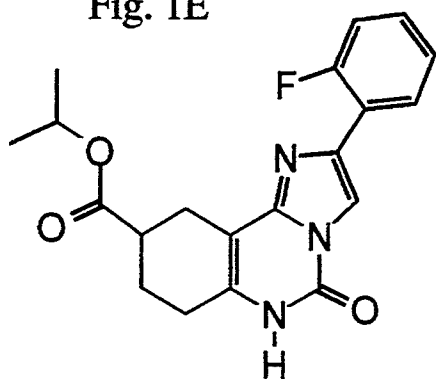
Compound 14
