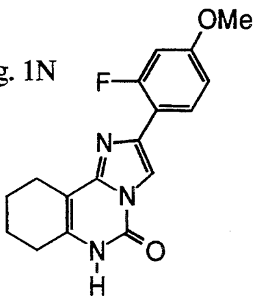
Compound 51
