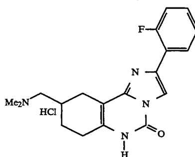
Compound 24
