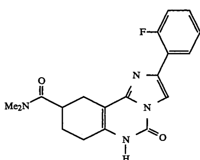
Compound 18
