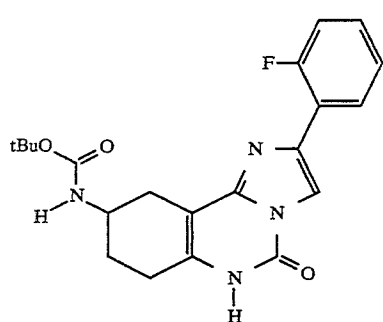
Compound 28 5
