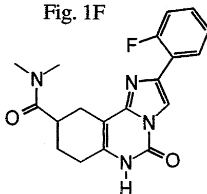
Compound 18
