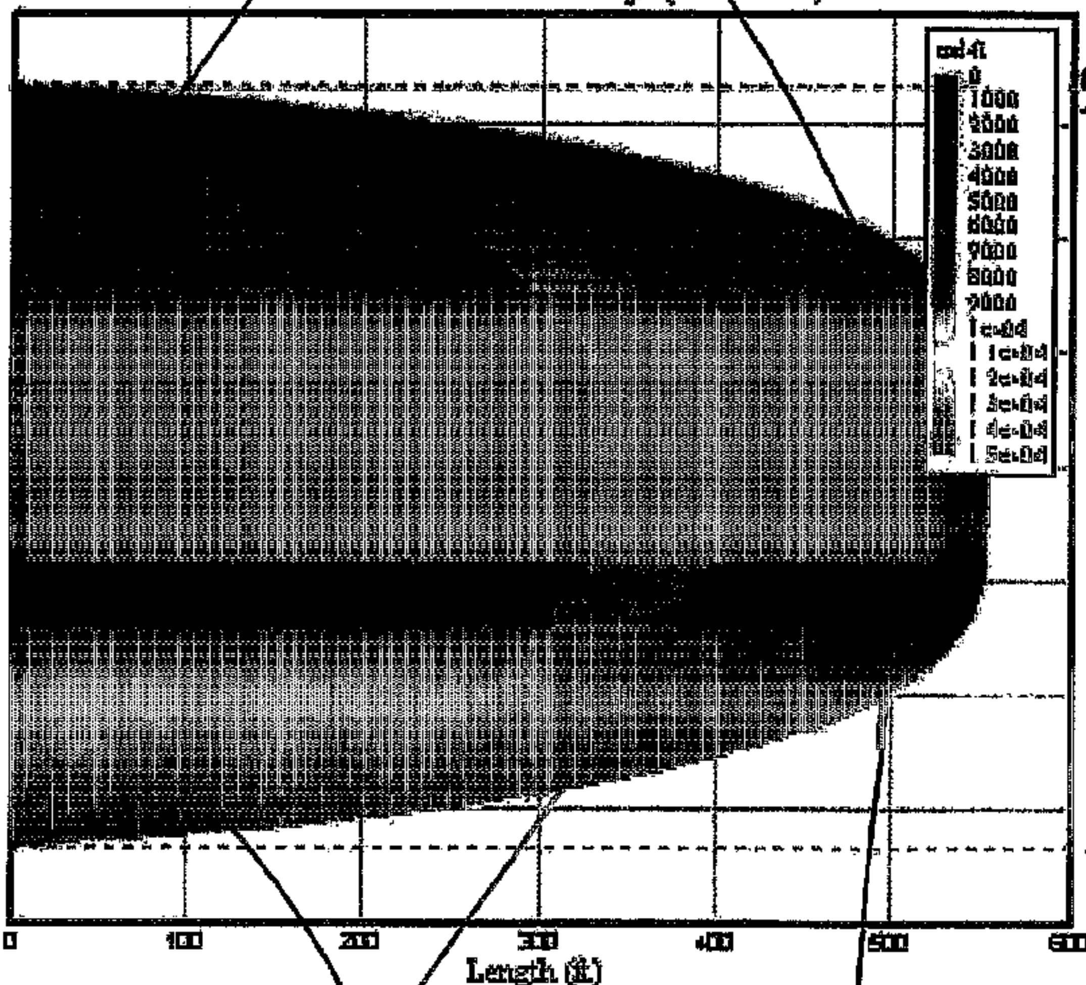
Fracture Conductivity (Closure)
