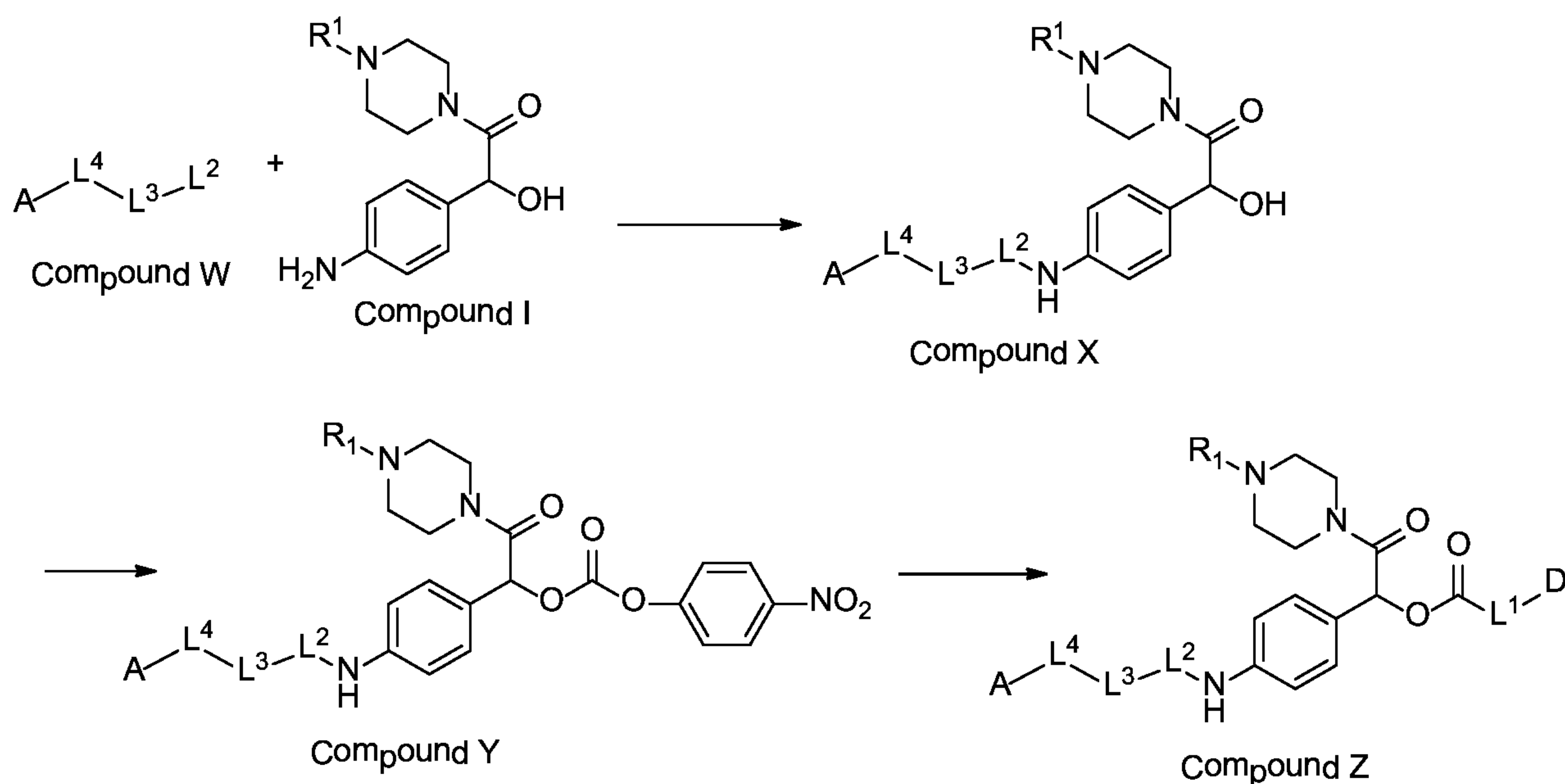
Scheme 4
