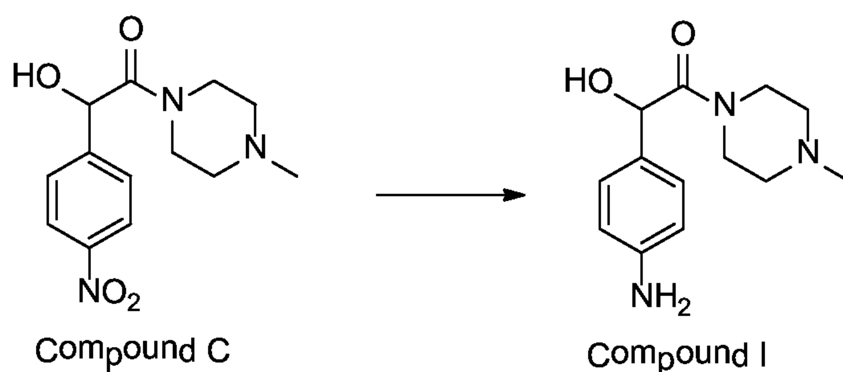
Scheme 3
