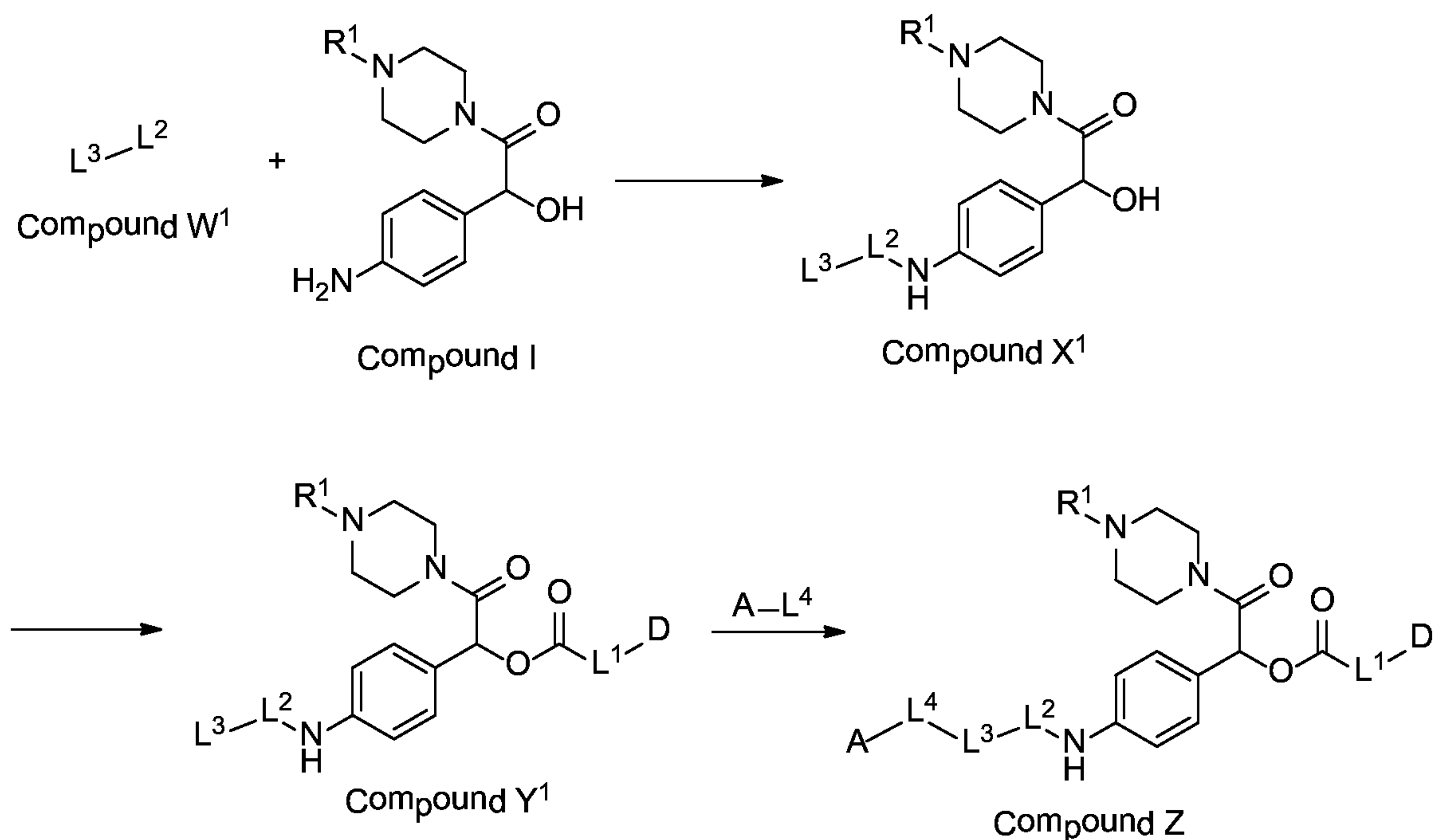
Scheme 5
