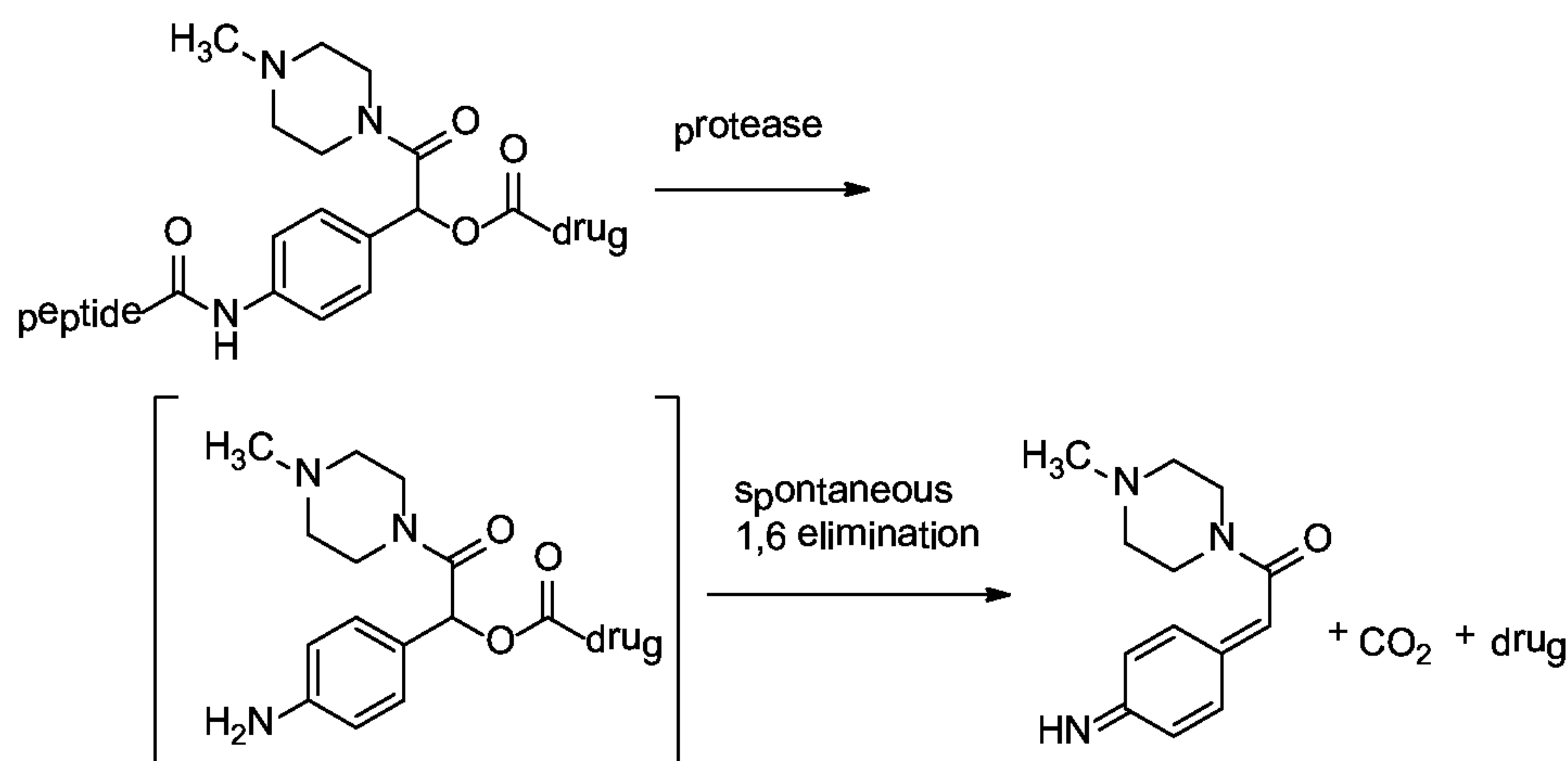
Scheme 1
