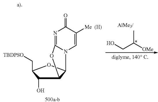
Scheme 8 2'-O-Alkyl Modifications
