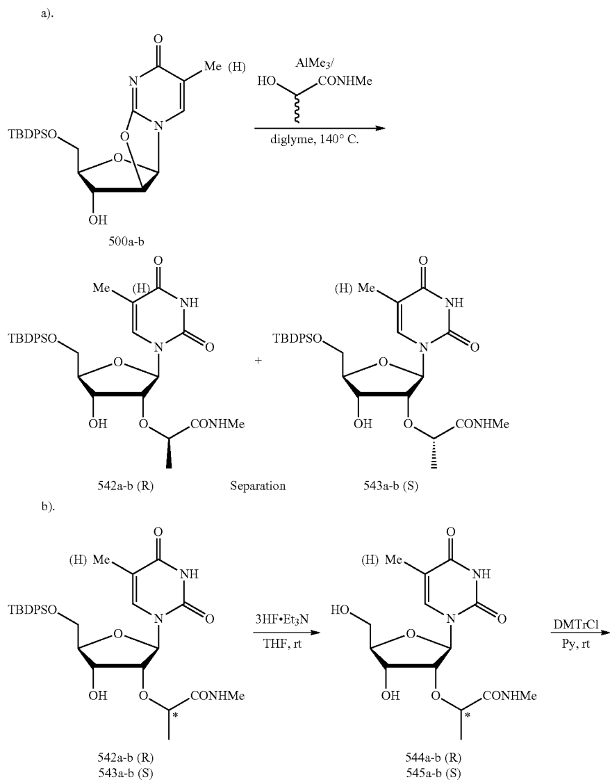
Scheme 12
