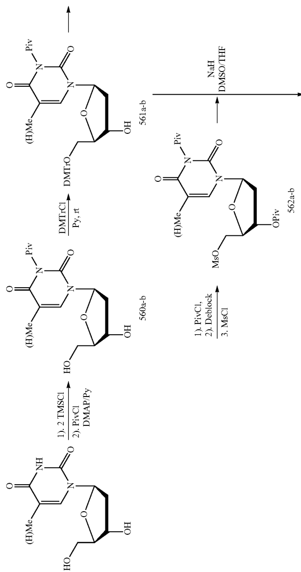
Scheme 15
