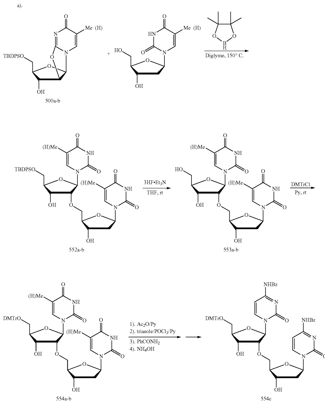
Scheme 13
