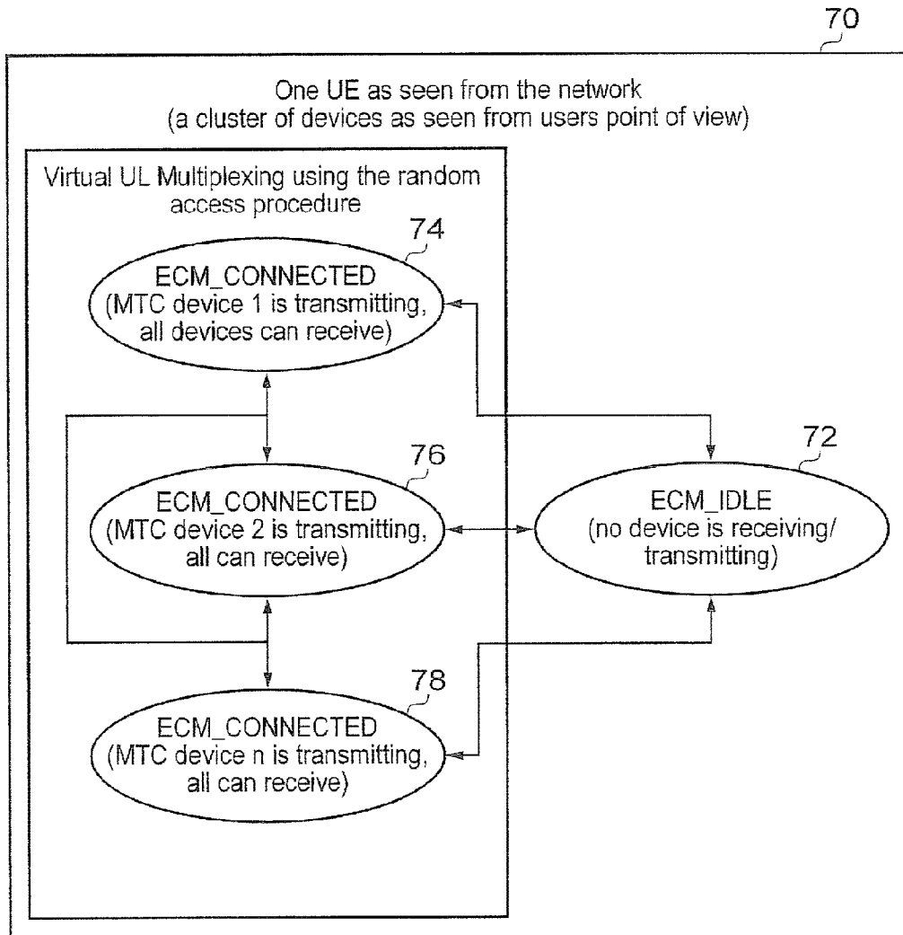
UL virtual multiplexing
