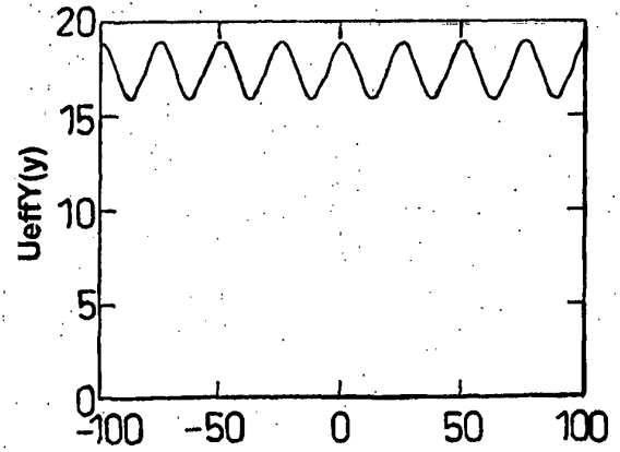
M = 200 at rf plates 3V ripple
