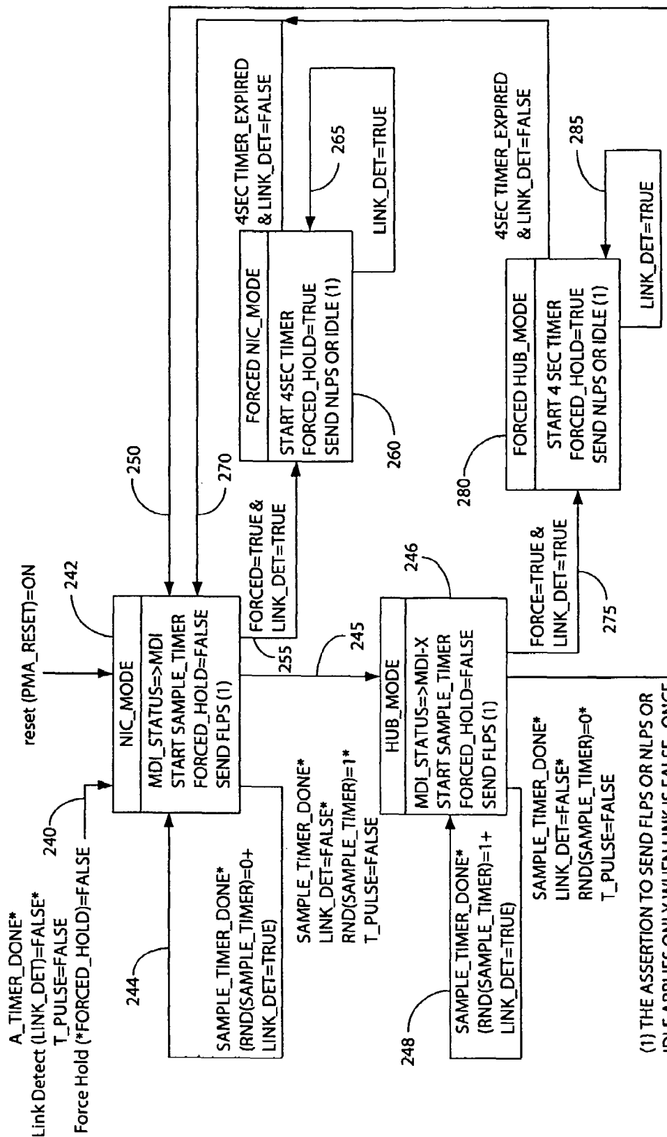
FIG. 5 FORCED MODE AUTO-MDIX STATE MACHINE
