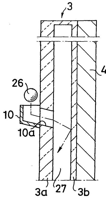
FIG. 4 (Sectional View of Transparent Game Board and LCD)
