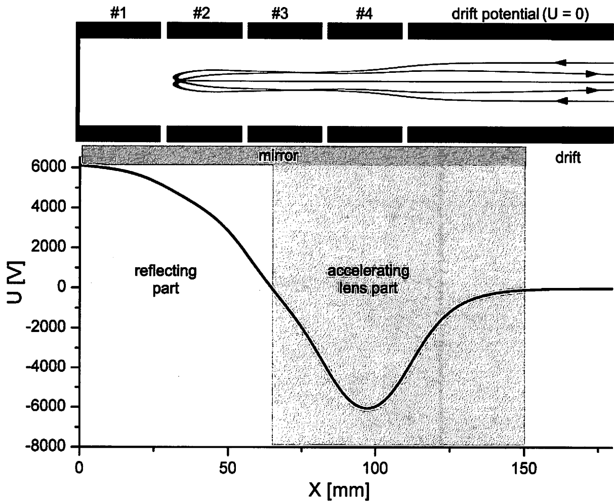
Fig. 1; Prior Art MPA-1
