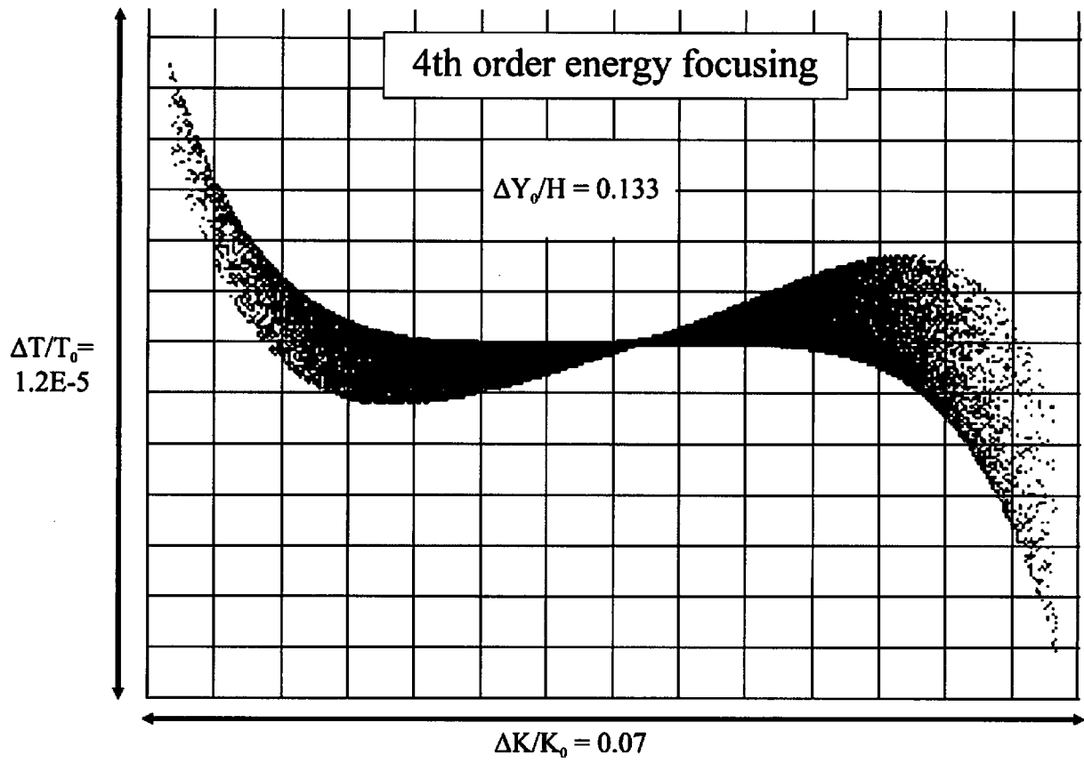
Fig. 6; Prior Art MPA-2-4
