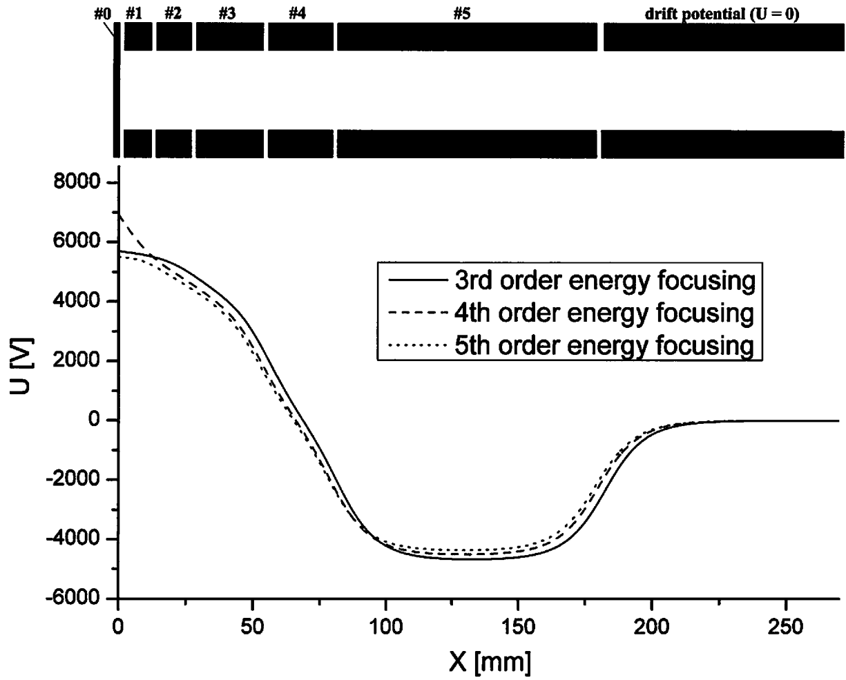
Fig. 3; Prior Art MPA-2
