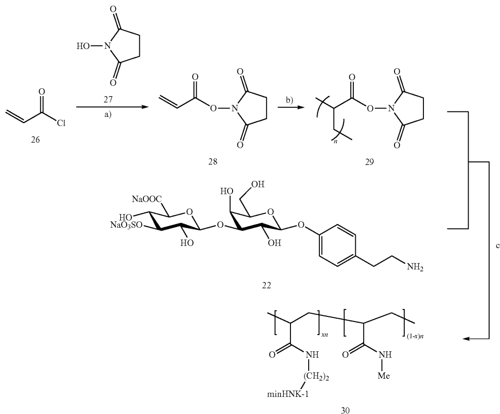
Scheme 3: Synthesis of the minimal HNK-1 polymer 30
