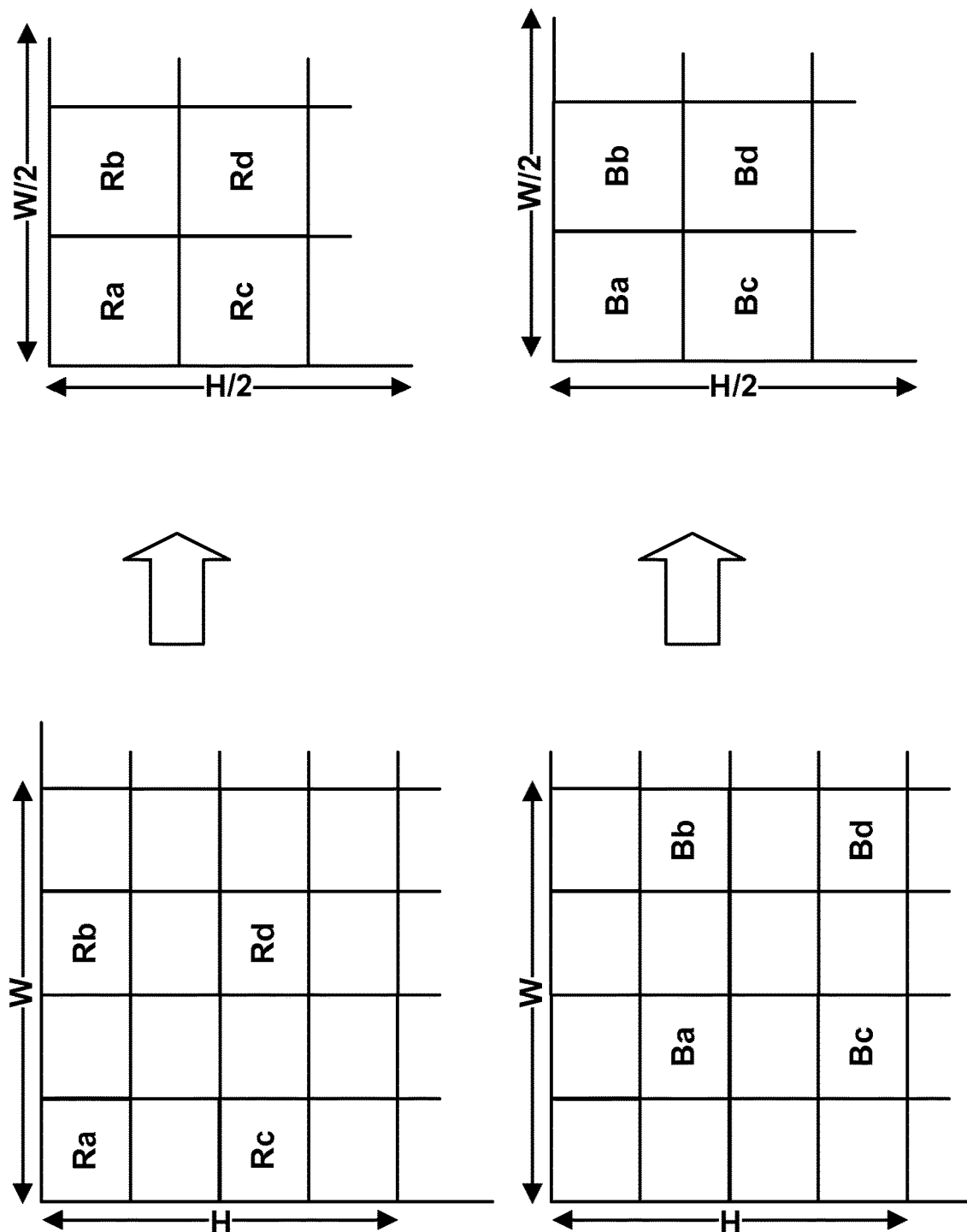
FIG. 2: Fast extraction of color primaries
