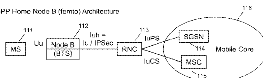
3GPP Home Node B (femto) Architecture
