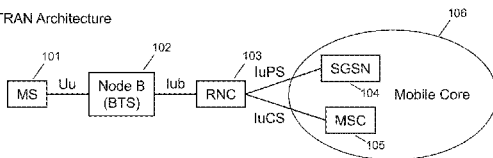
3GPP UTRAN Architecture
