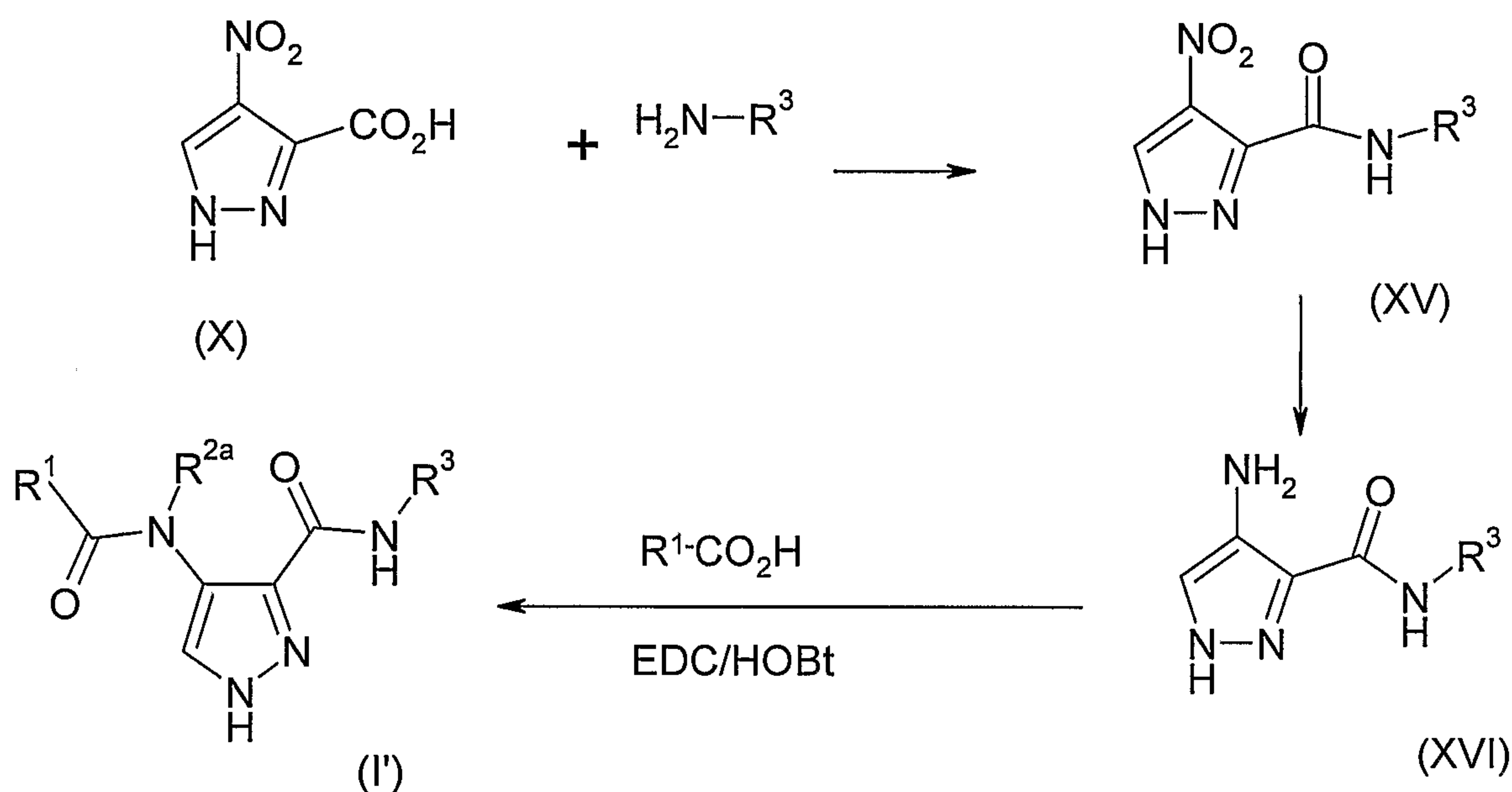
Scheme 2
