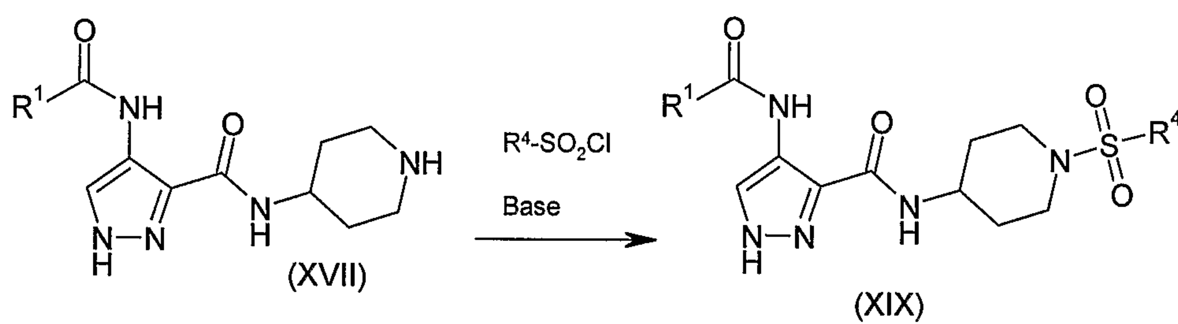
Scheme 3
