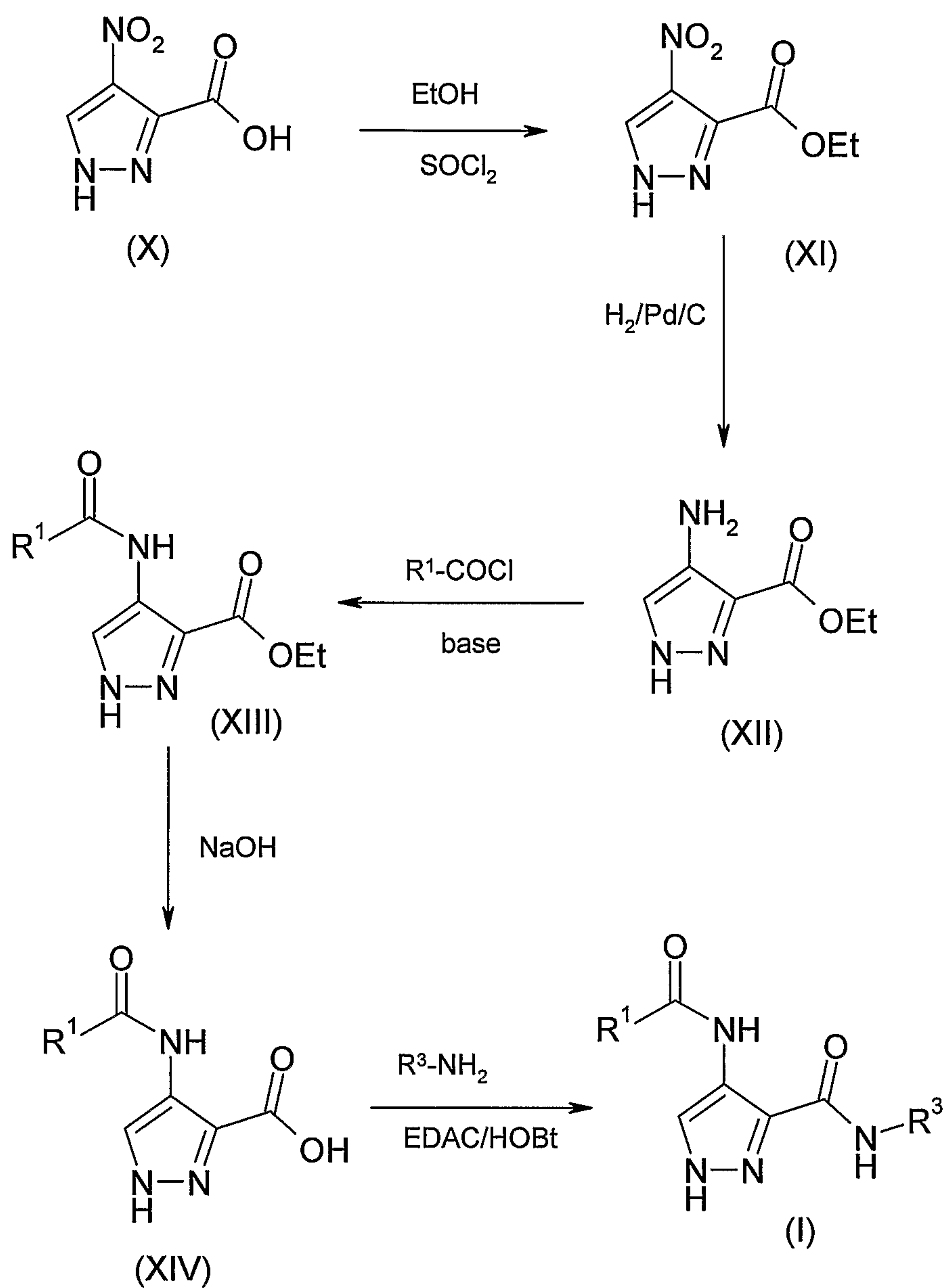
Scheme 1
