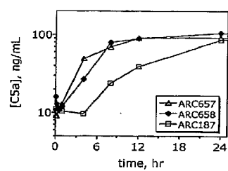
Figure 43c [CSa] vs time
