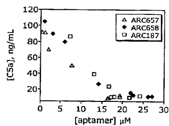
Figure 43d [CSa] vs [aptamer]
