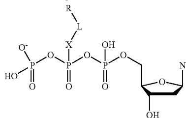
beta-modified dNTPs
