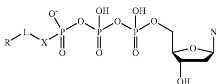
gamma-modified dNTPs
