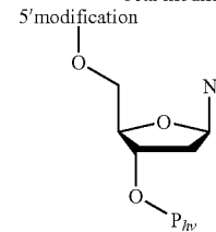
Modification at the 3' position P_{hv} is a photolabile group linked to the 3'-O
