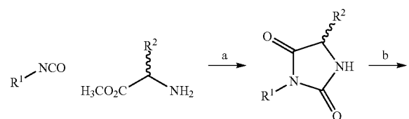
Scheme 3: Synthesis of cyclic urea hydroxamic acids
