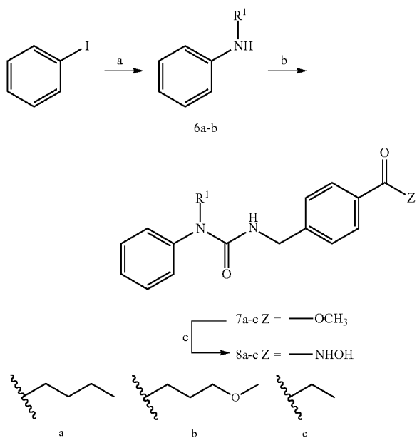
Scheme 2: Synthesis of distal N-substituted hydroxamic acids
