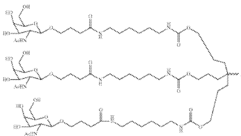
Formula XB
