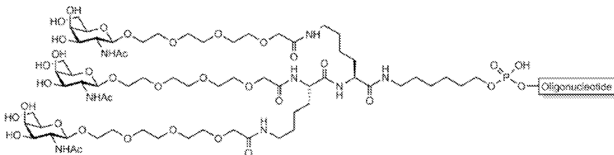
Formula XE
