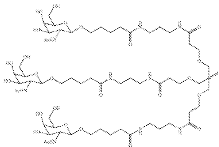
Formula XA
