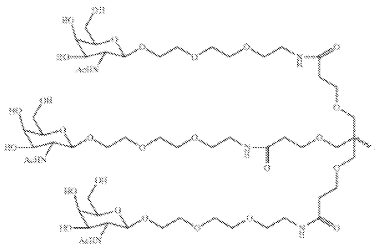
Formula XC
