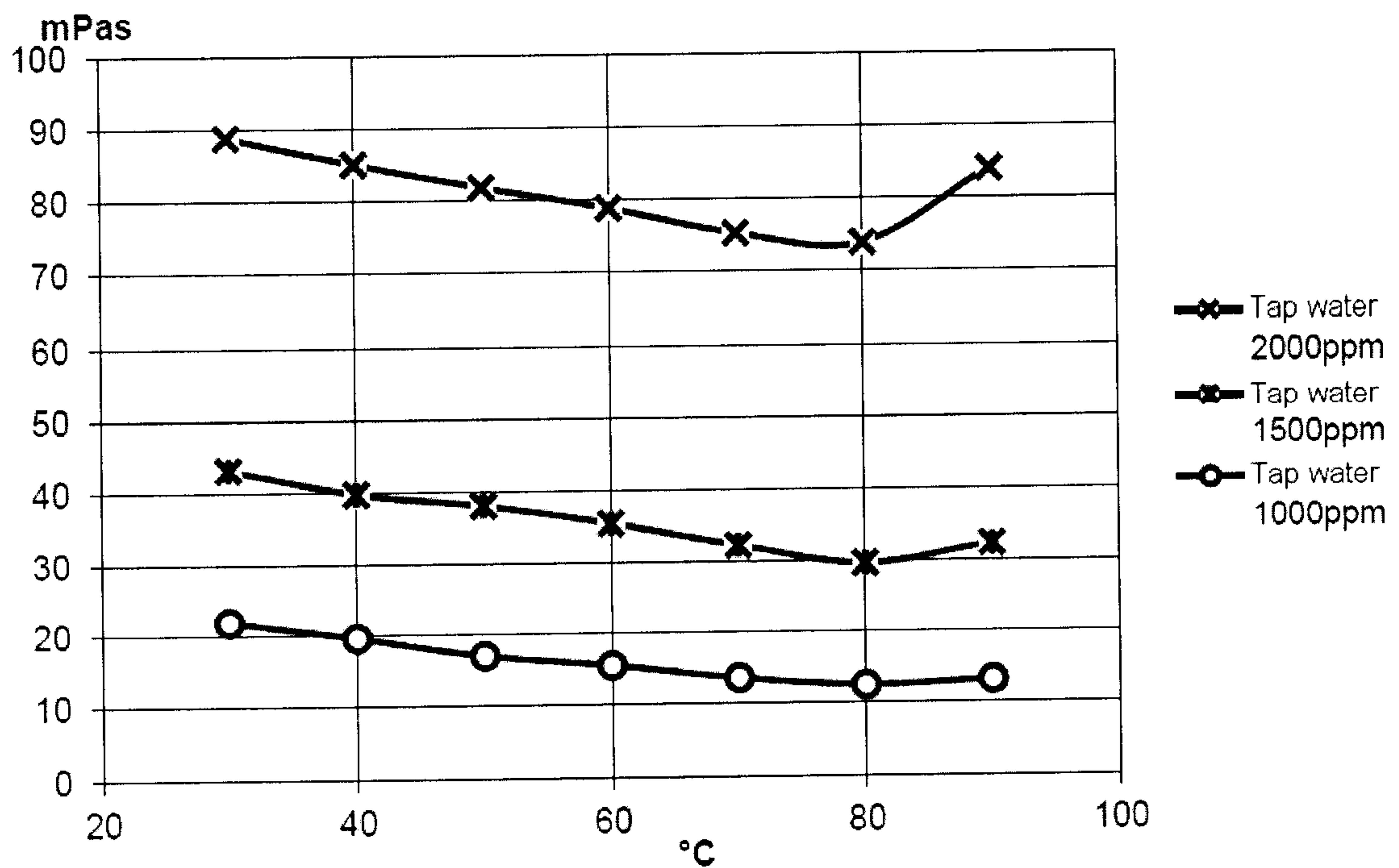
Figure 6b: Viscosity of solutions of copolymer 4 in tap water at various temperatures and concentrations.
