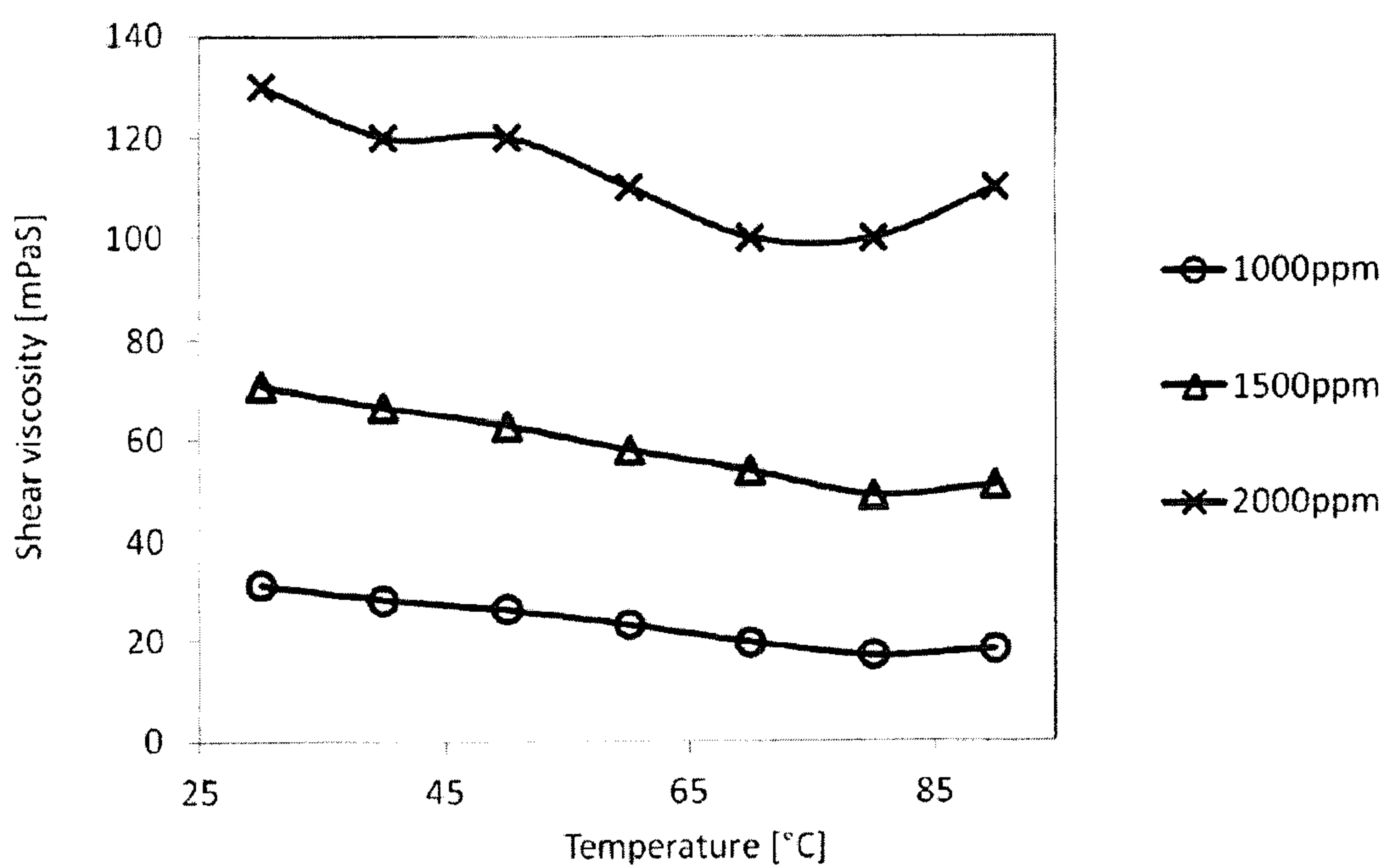
Figure 10b: Viscosity of solutions of copolymer V5 in tap water at various temperatures and concentrations
