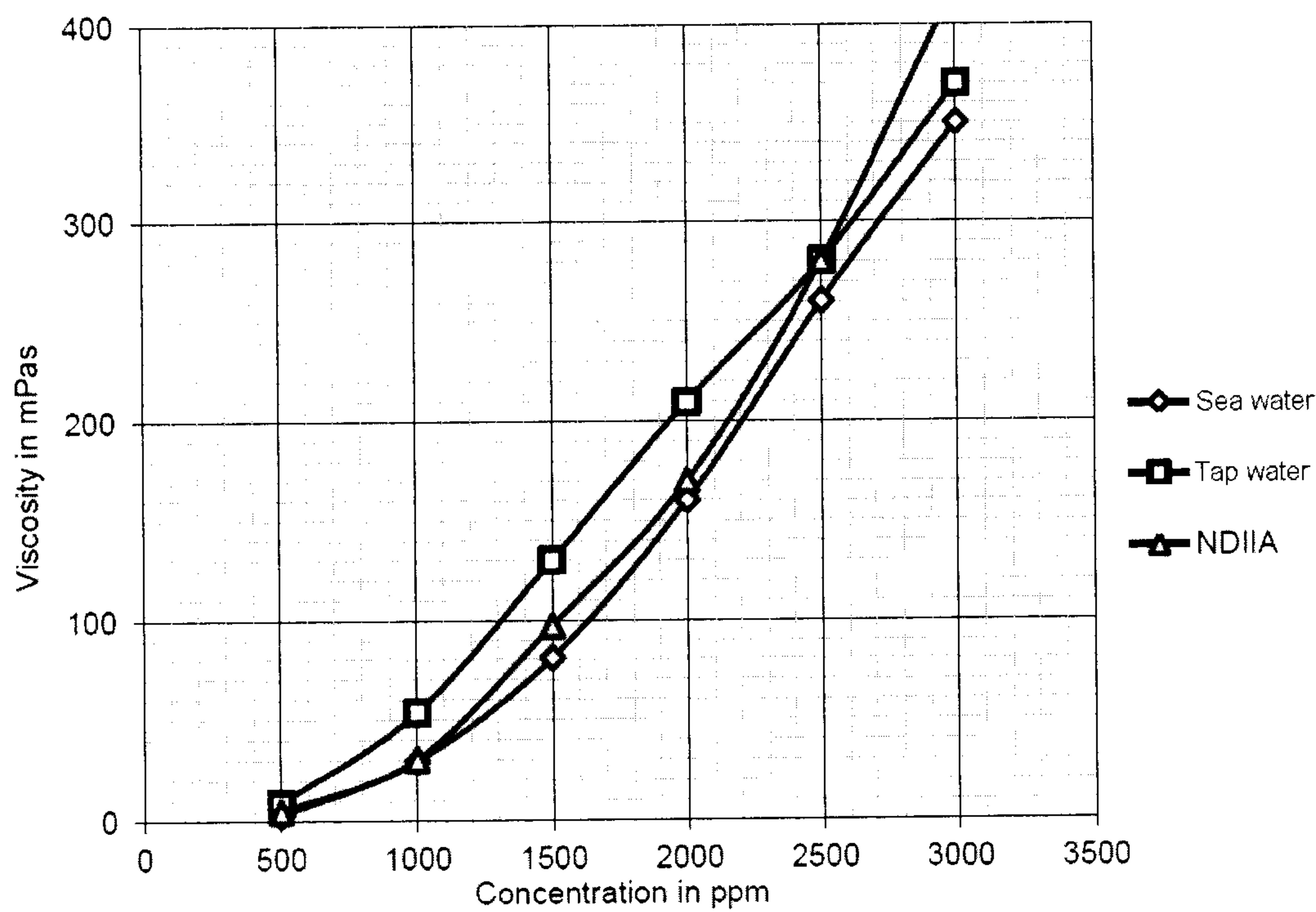
Figure 4a: Viscosity of copolymer 2 at 60°C at various concentrations in seawater, tap water and deposit water.
