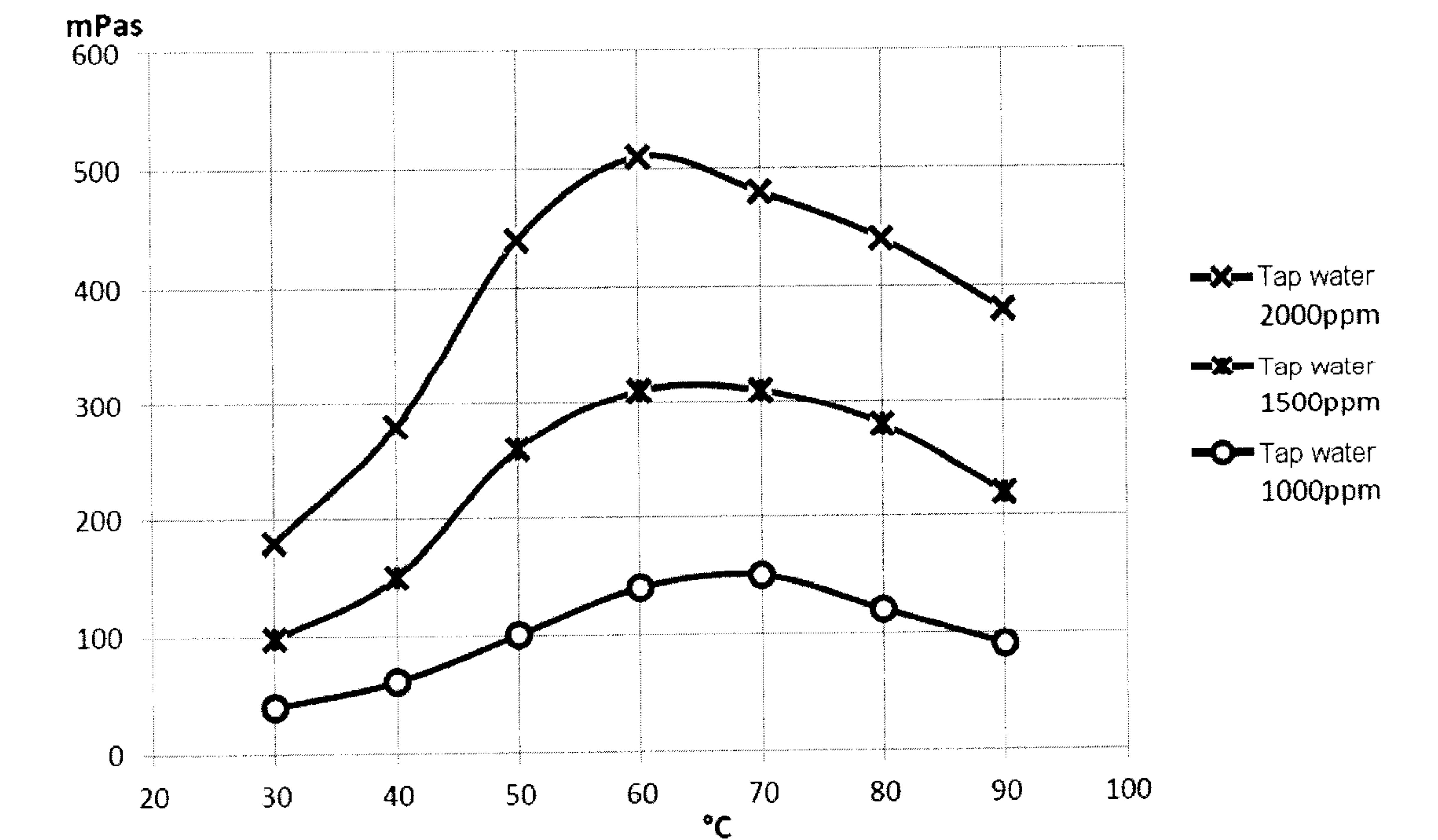
Figure 2b: Viscosity of aqueous solutions of copolymer V2 in tap water at various temperatures and concentrations.
