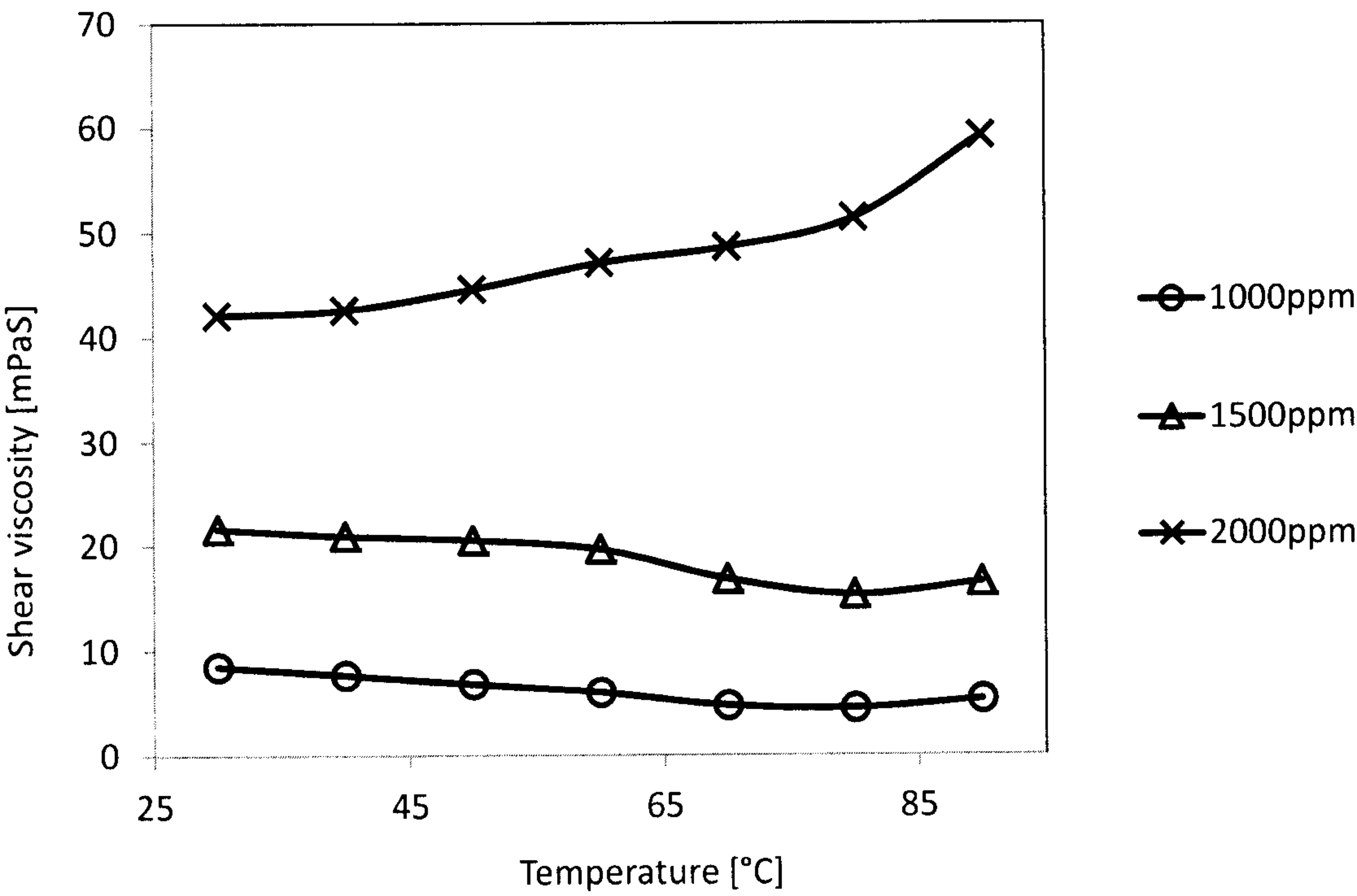
Figure 10c: Viscosity of solutions of copolymer V5 in sea water at various temperatures and concentrations
