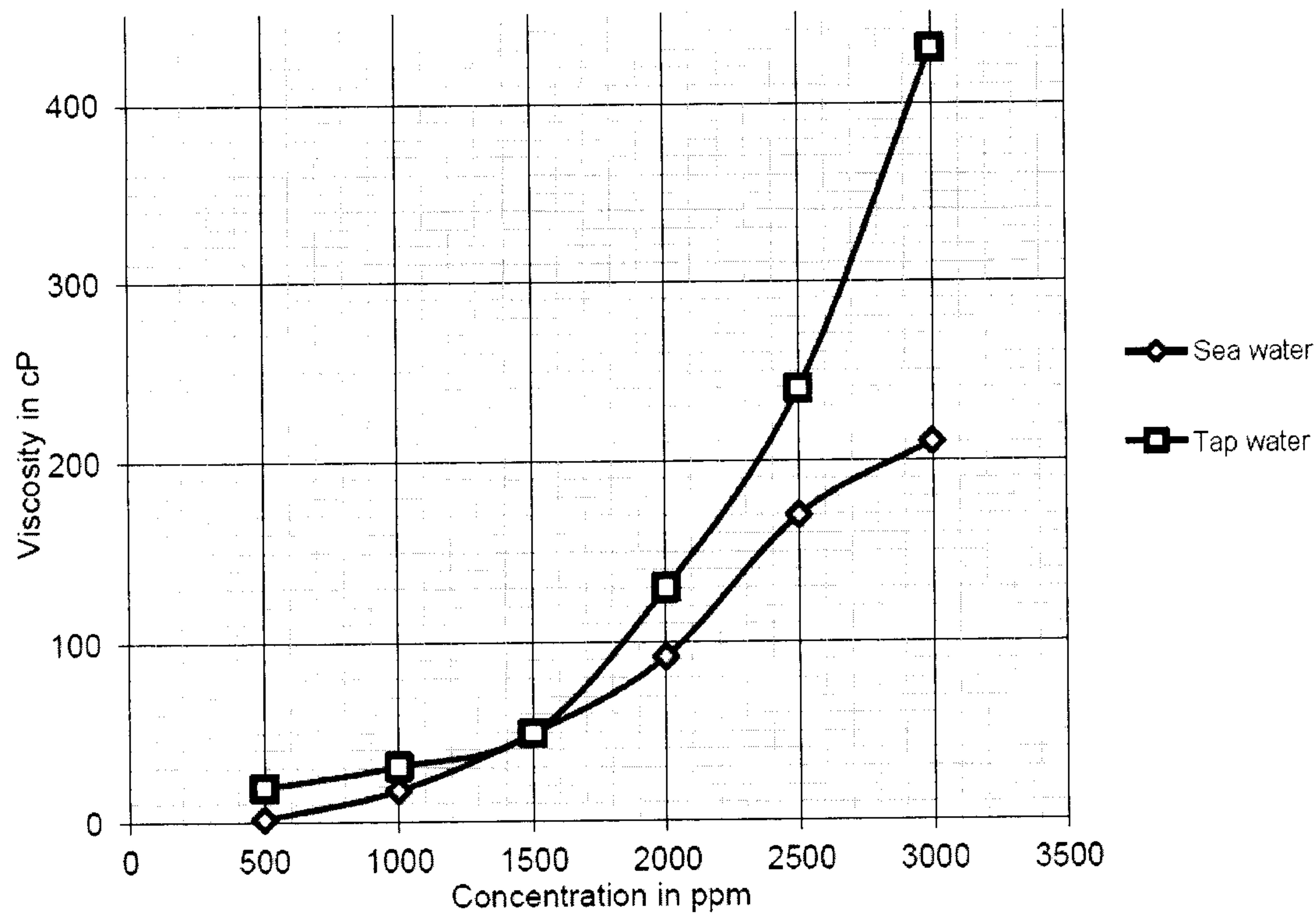
Figure 7a: Viscosity of copolymer 5 at 60°C at various concentrations in seawater and tap water.
