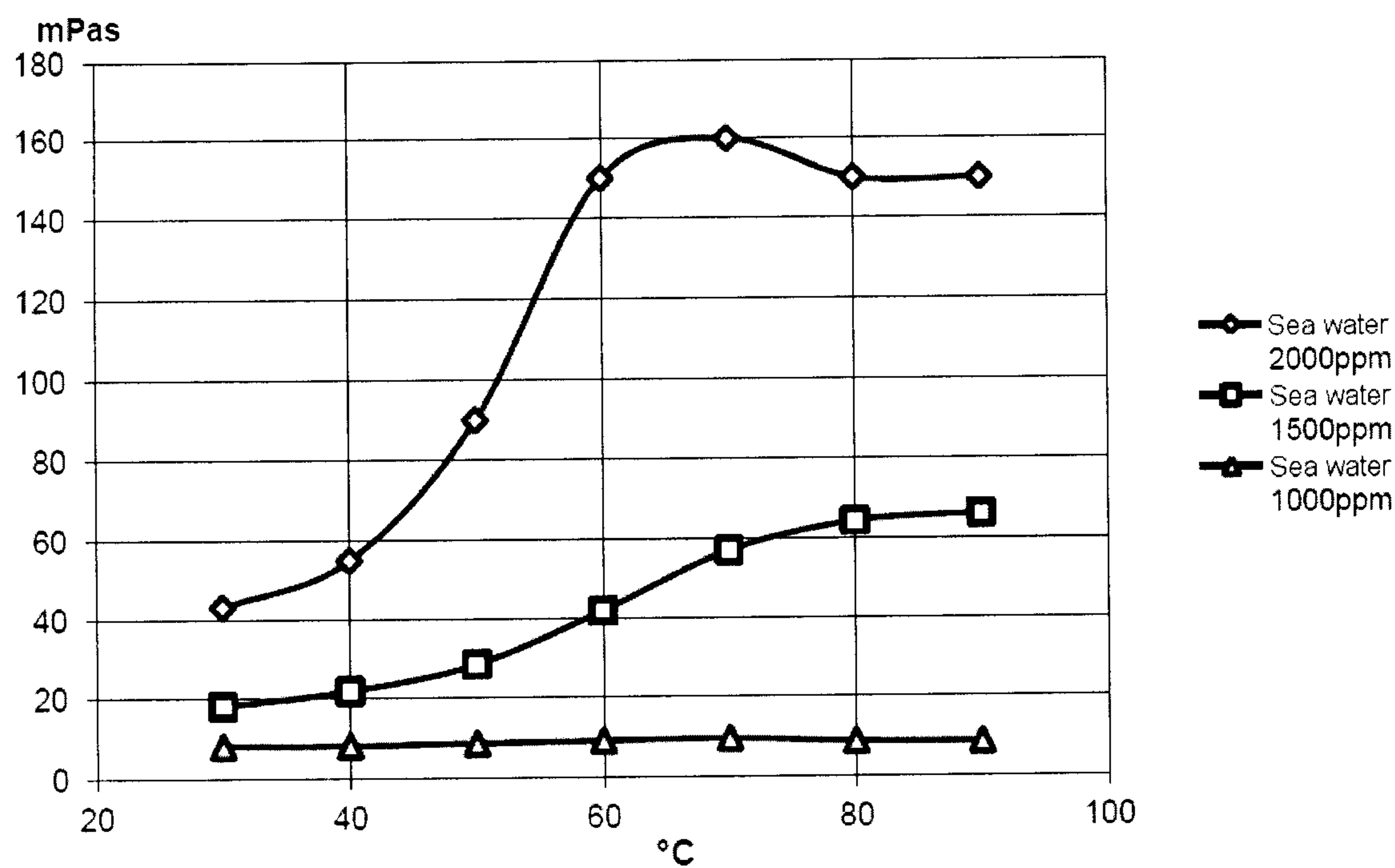
Figure 5c: Viscosity of solutions of copolymer 3 in seawater at various temperatures and concentrations.
