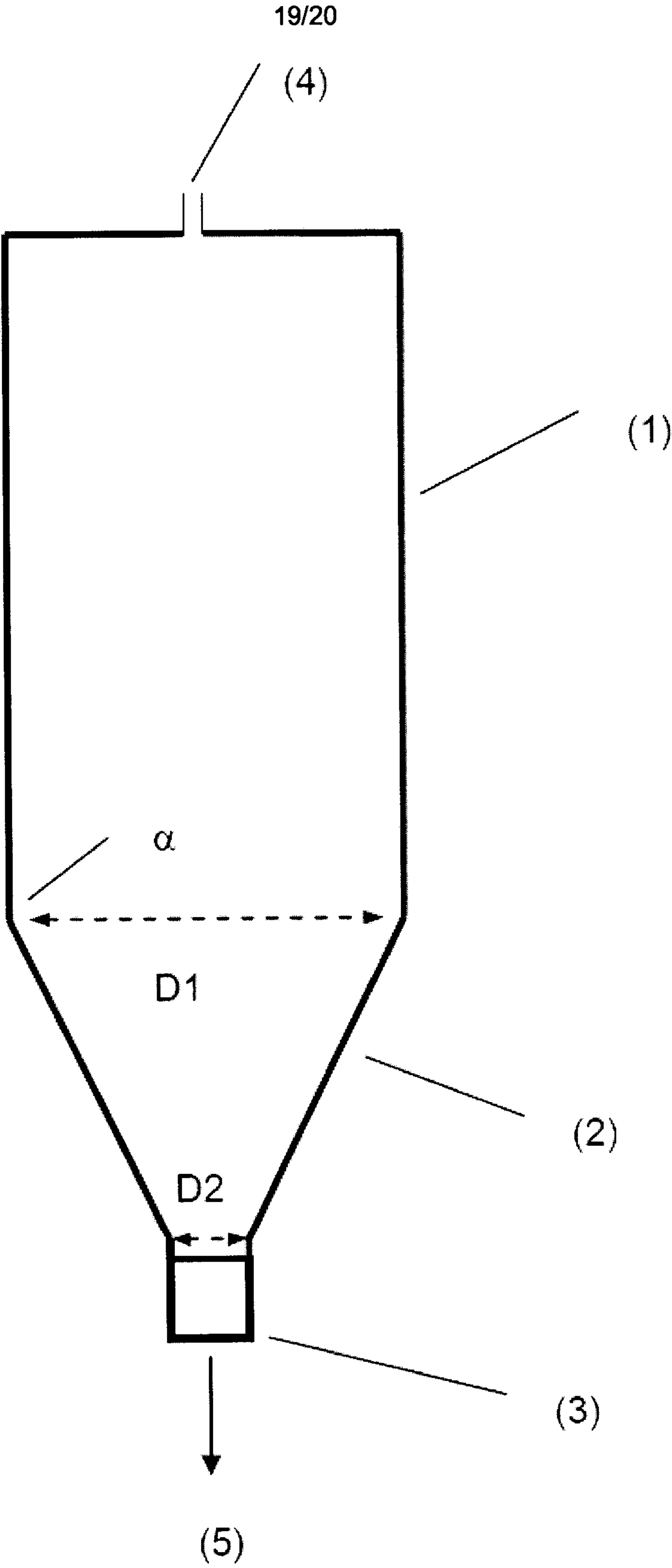
Figure 11: Partly conical reactor
