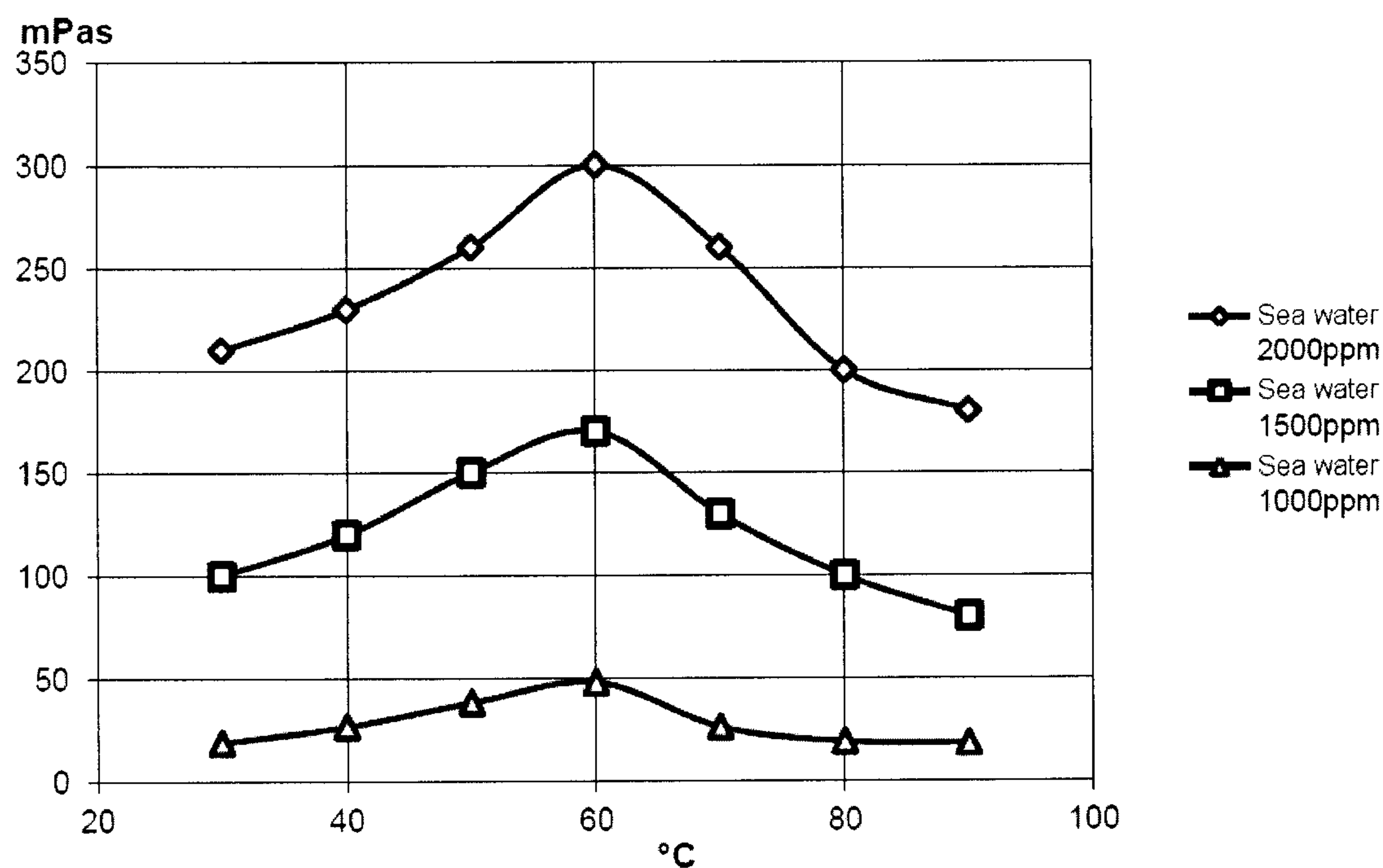
Figure 2c: Viscosity of solutions of copolymer V2 in seawater at various temperatures and concentrations.
