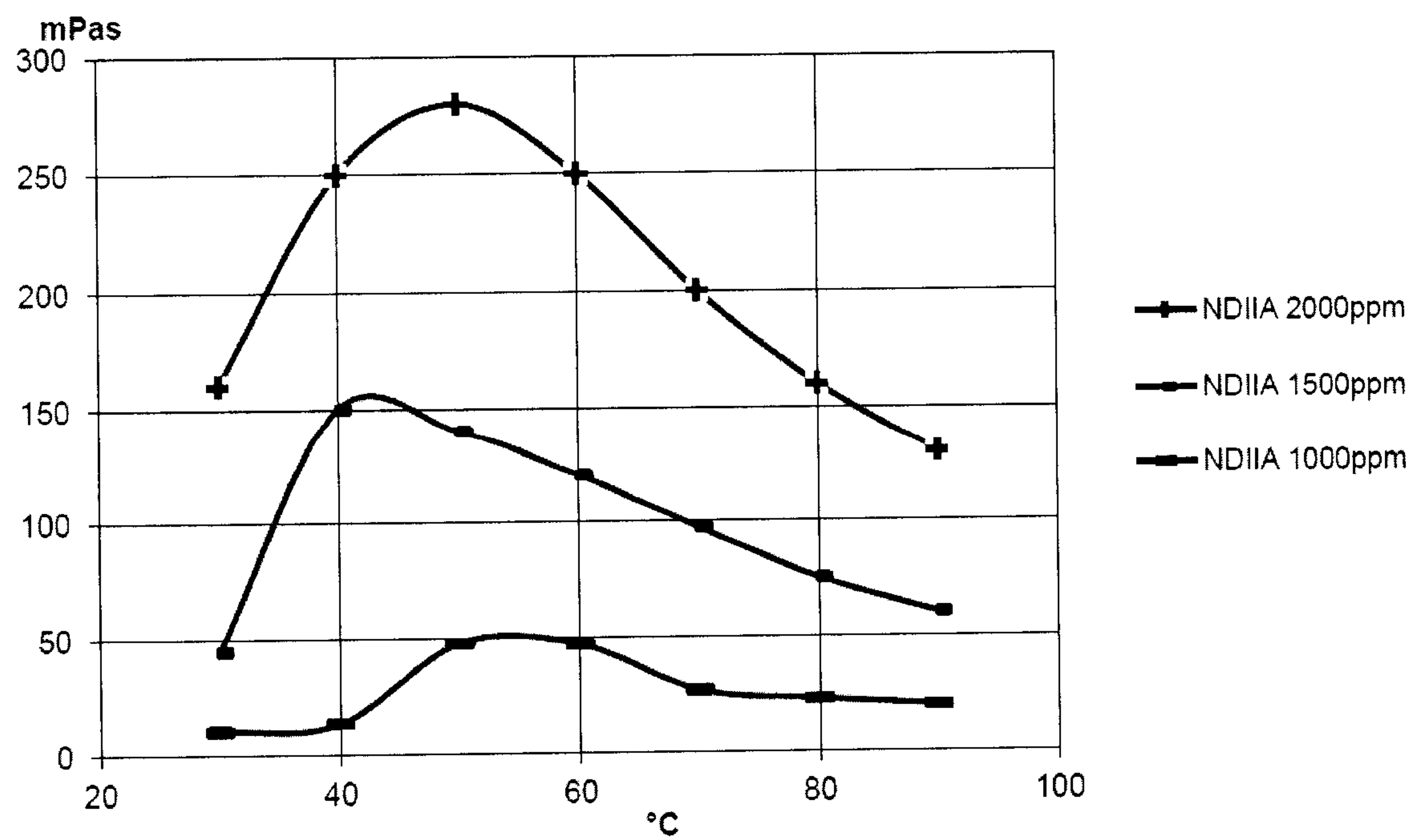
Figure 5d: Viscosity of solutions of copolymer 3 in deposit water at various temperatures and concentrations.
