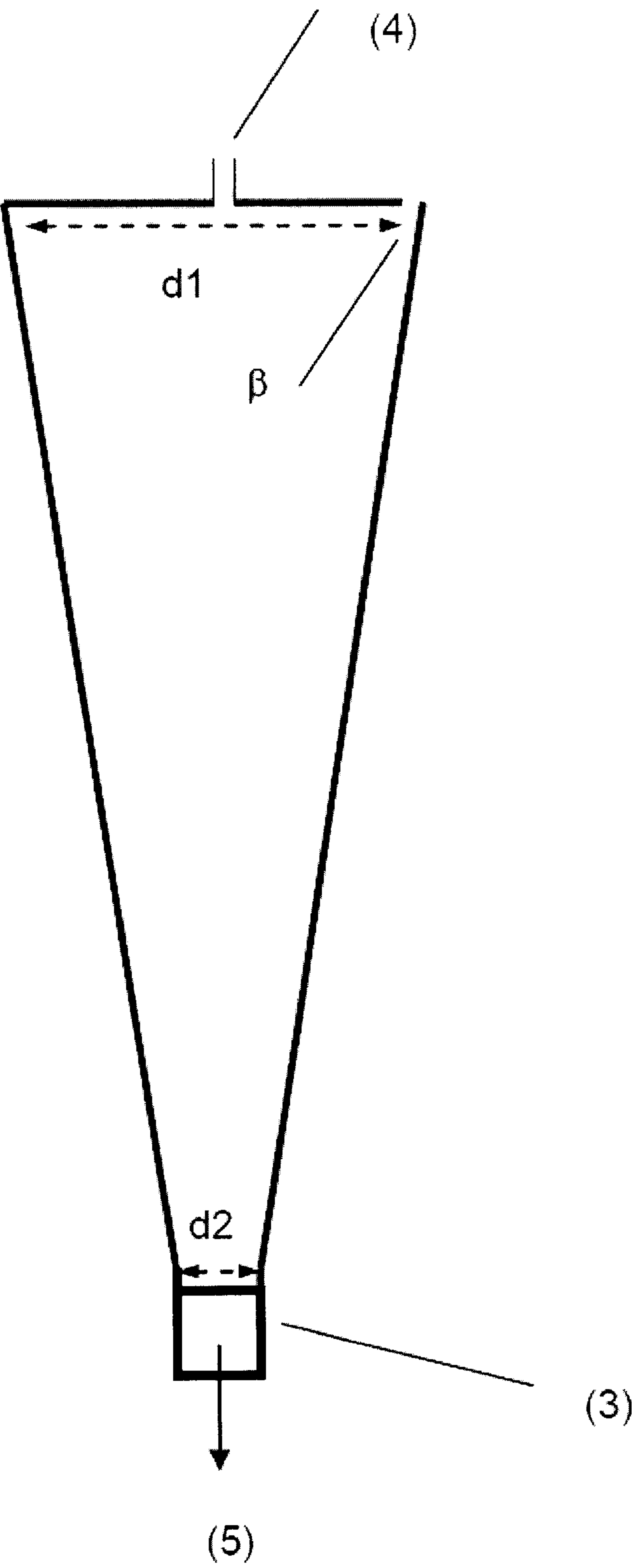
Figure 12: Fully conical reactor
