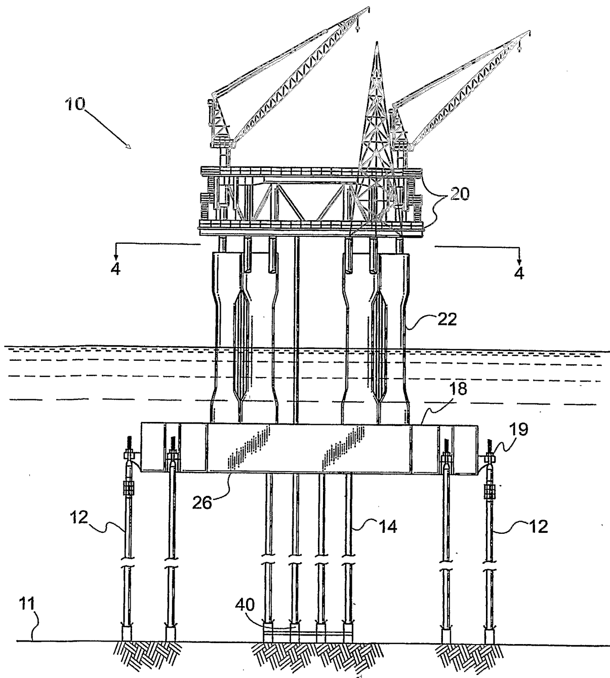
Fig. 3 (Prior Art)
