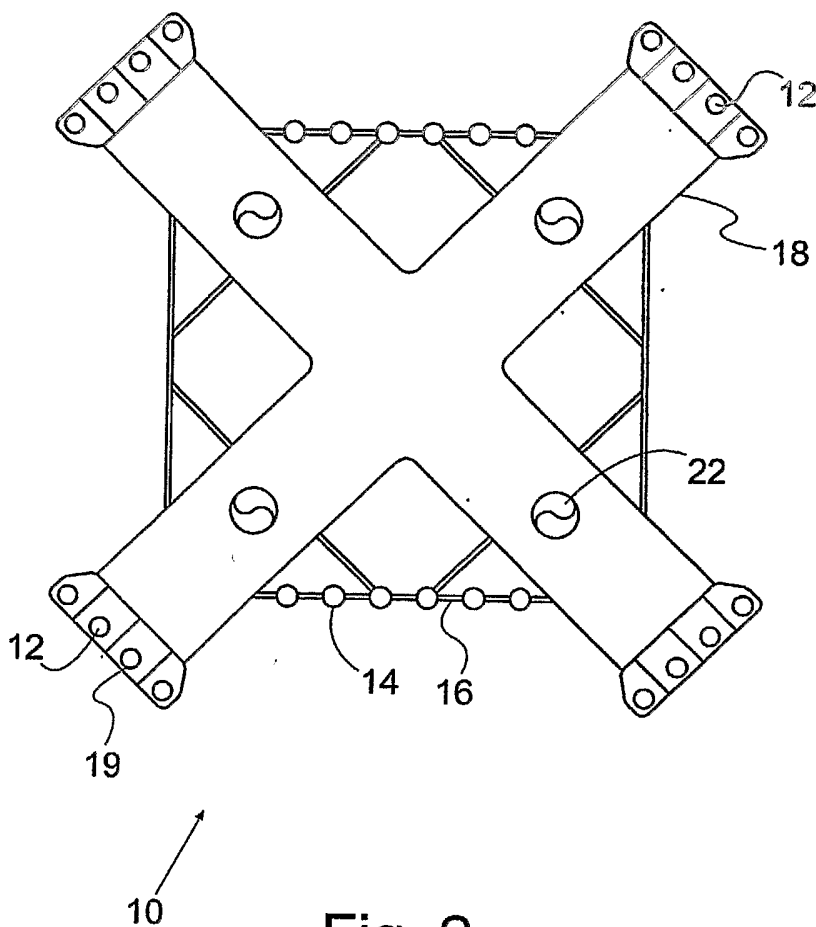
Fig. 2 (Prior Art)
