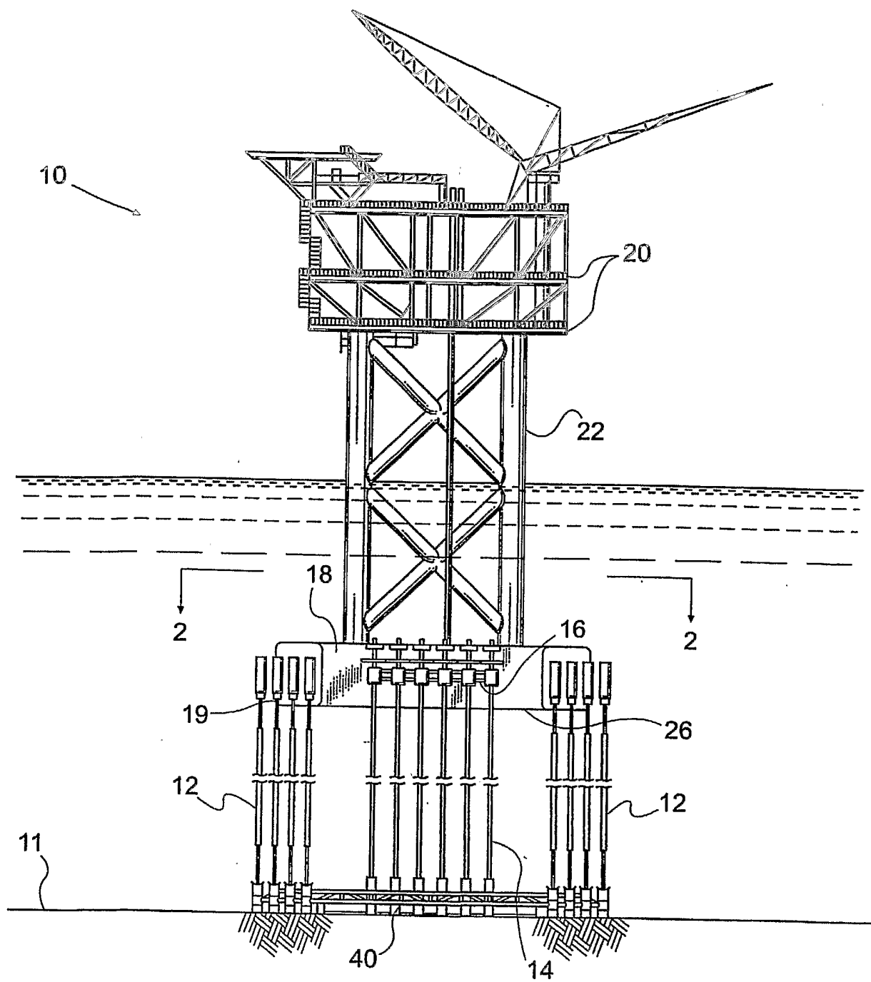
Fig. 1 (Prior Art)
