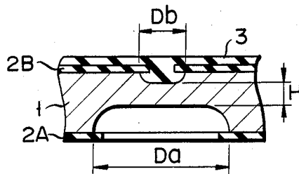
FIG. 2 (PRIOR ART)
