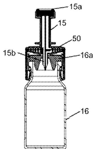
Fig. 5a PRIOR ART
