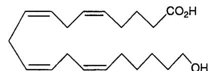
14,15-Dehydro-20-HETE (26)
