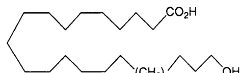
20-Hydroxyeicosanoic Acid (55: n = 1)
