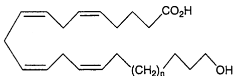
19-Hydroxynonadeca-5(Z),8(Z),11(Z),14(Z)-tetraenoic Acid (9a: n = 0)
