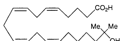
20,20-Dimethyl-20-HETE (19)
