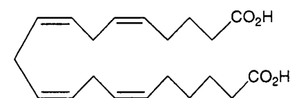
Eicosatetraen-1,20-dioic Acid
