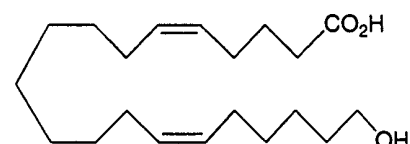
20-Hydroxyeicosa-5(Z),14(Z)-dienoic Acid (50)
