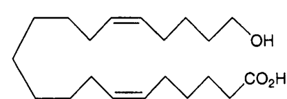
20-Hydroxyeicosa-6(Z),15(Z)-dienoic Acid (54)
