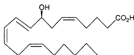
8(S)-HETE
