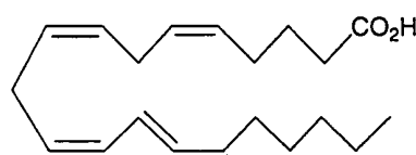
15(S)-HETE
