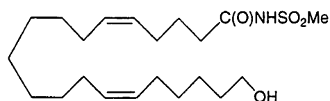
N-Methylsulfonyl-20-Hydroxyeicosa-5(Z),14(Z)-dienamide
