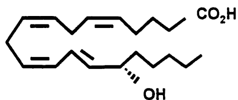
15(S)-HETE
