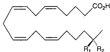
19(S)-HETE (34: R 1 = H, R 2 = OH)
