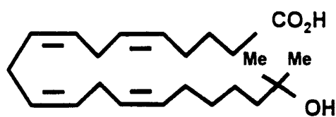
Dimethyl 20-HETE
