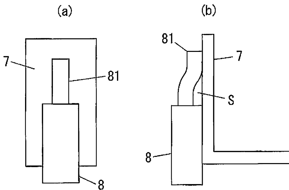
FIG. 8 (PRIOR ART)
