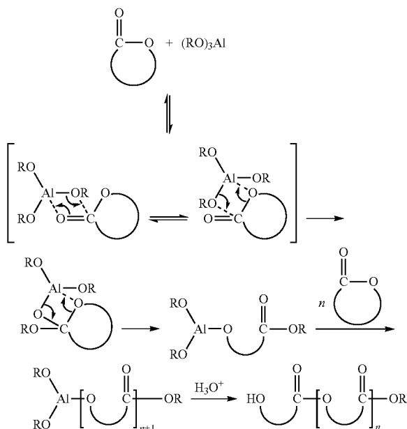
Diagram 5: Polymerization mechanism by coordination-insertion
