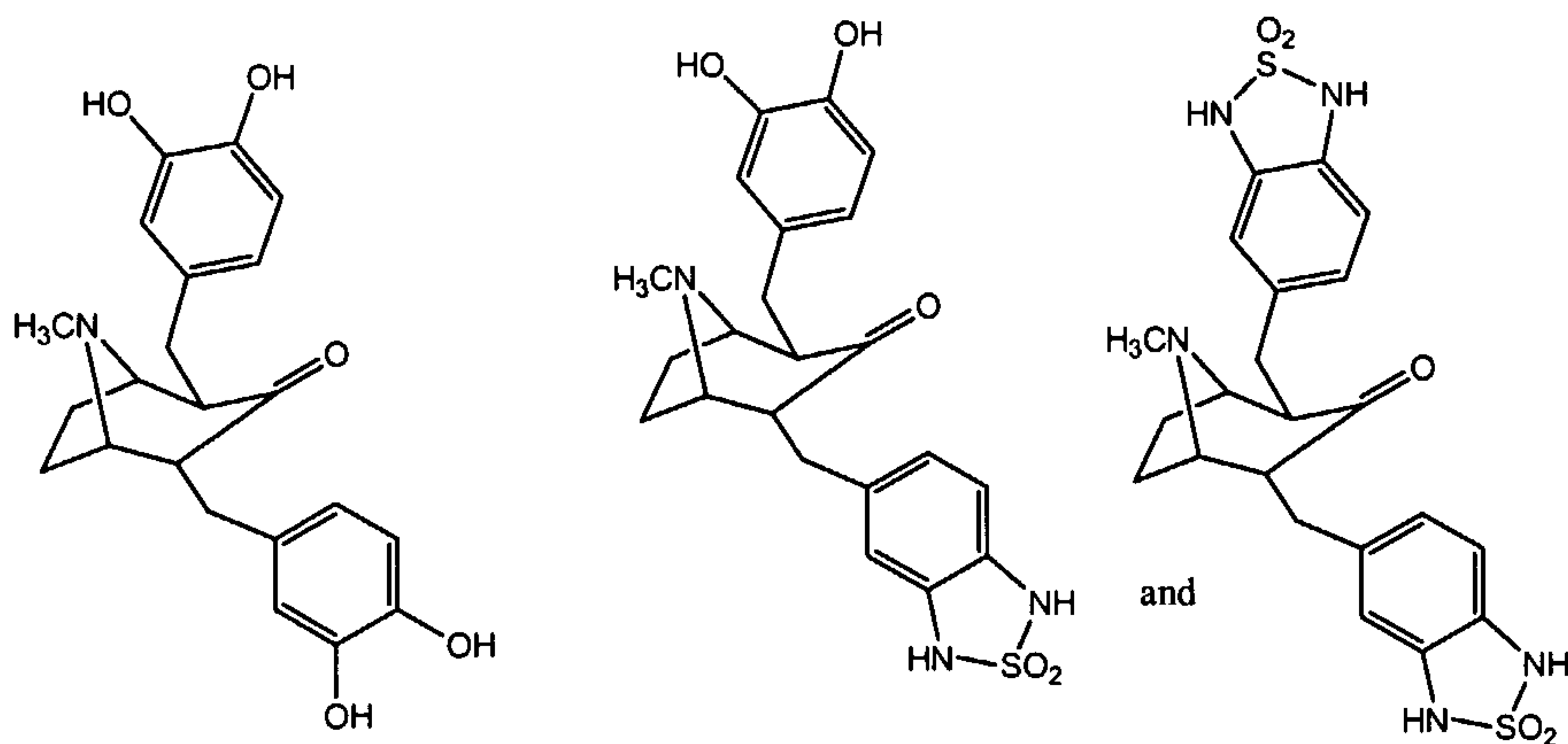
2,4-bis(3,4-dihydroxybenzyl)-8-methyl-8-aza-bicyclo[3.2.1]octan-3-one
