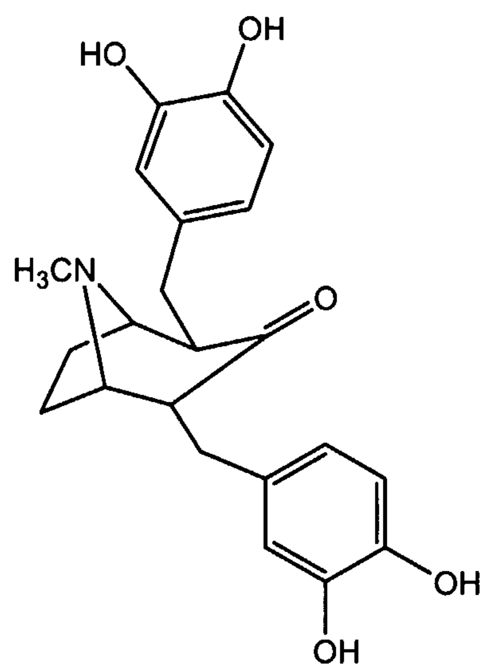
2,4-bis(3,4-dihydroxybenzyl)-8-methyl -8-aza-bicyclo[3.2.1]octan-3-one
