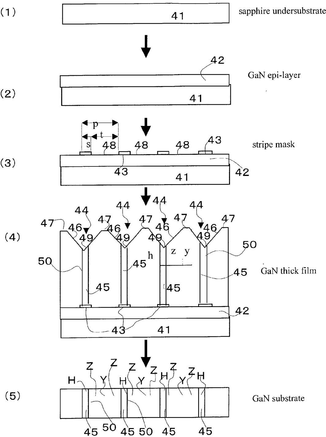
Fig. 10 Processes of producing a GaN substrate
