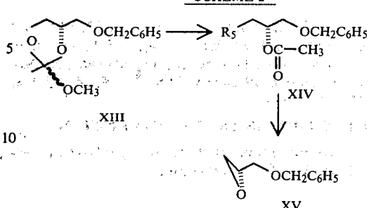
-continued SCHEME 2
