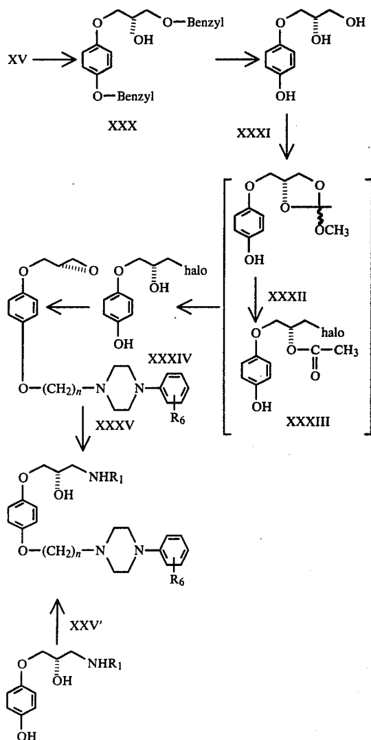
SCHEME 4
