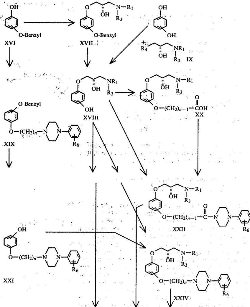
SCHEME 3
