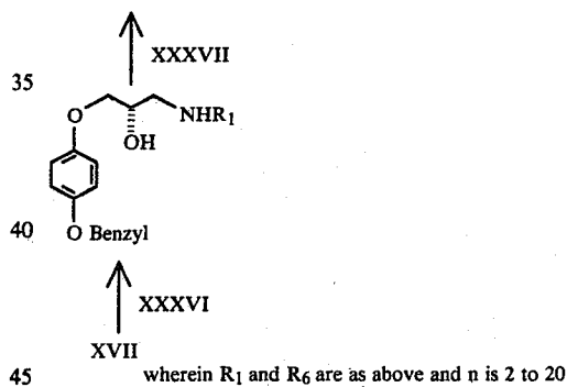
-continued SCHEME 4
