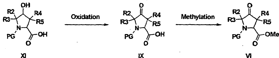
Scheme 5
