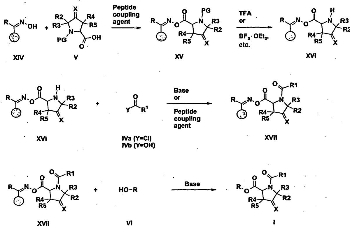
Scheme 8
