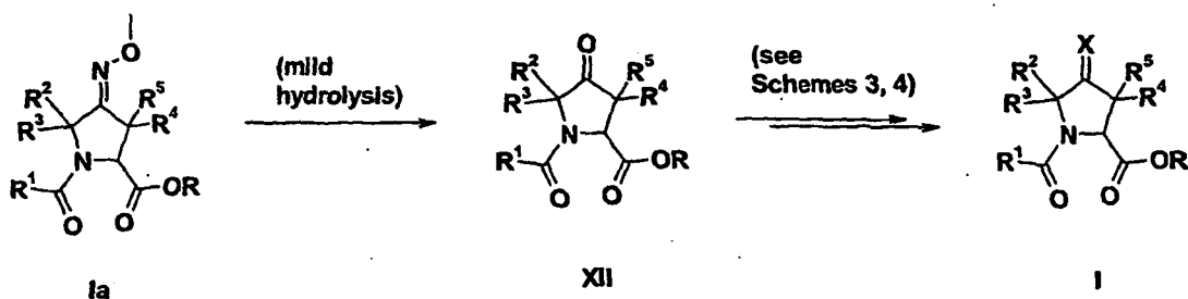
Scheme 6
