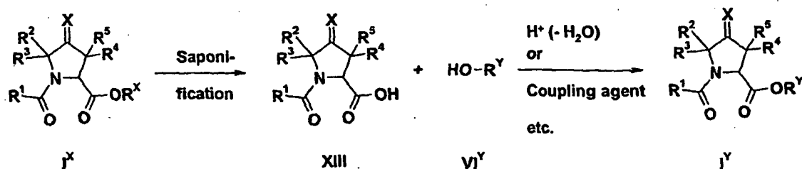
Scheme 7
