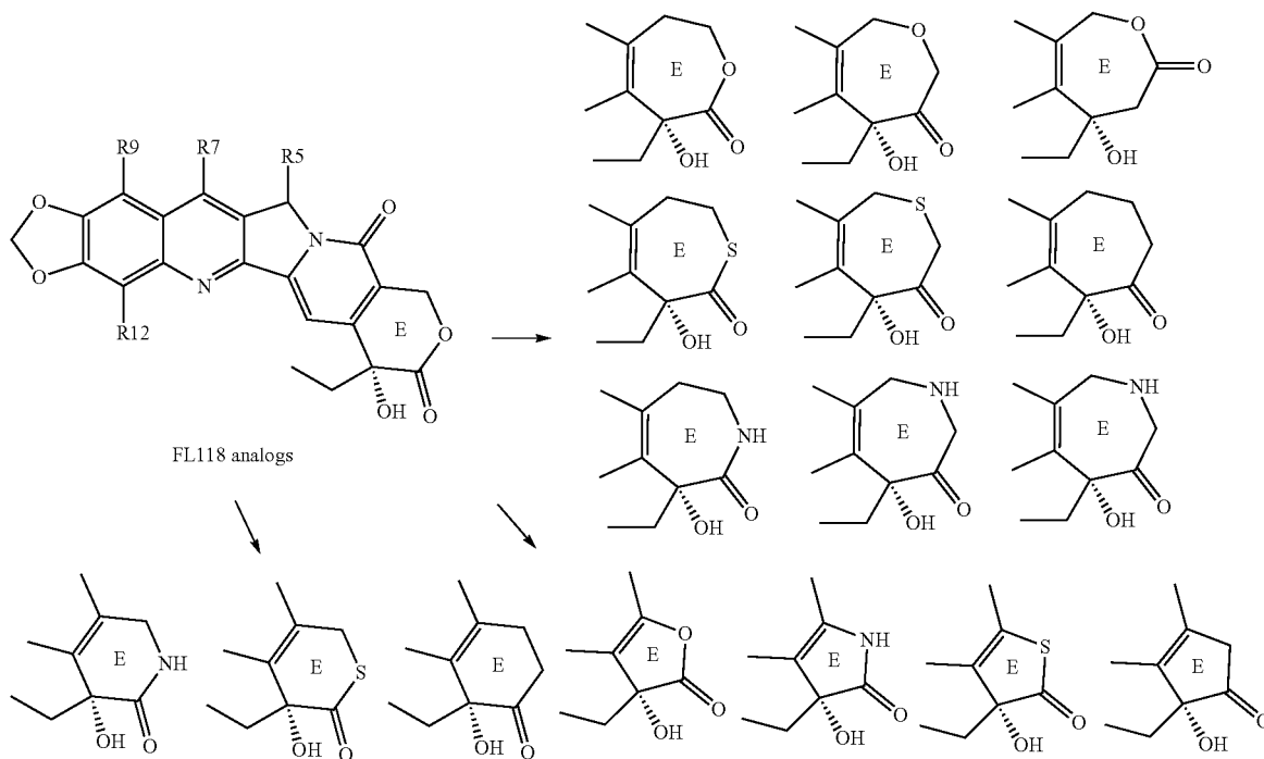
Scheme 3: Modification of the E-ring structure
