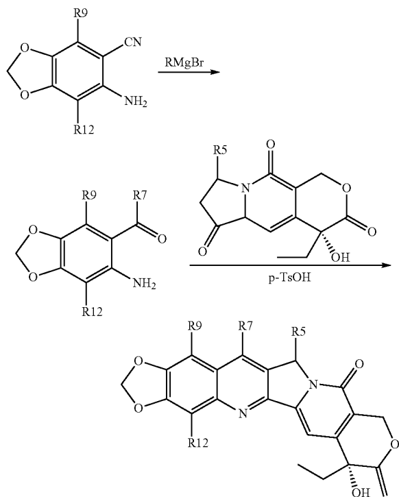
Scheme 2: FL118 analog synthesis
