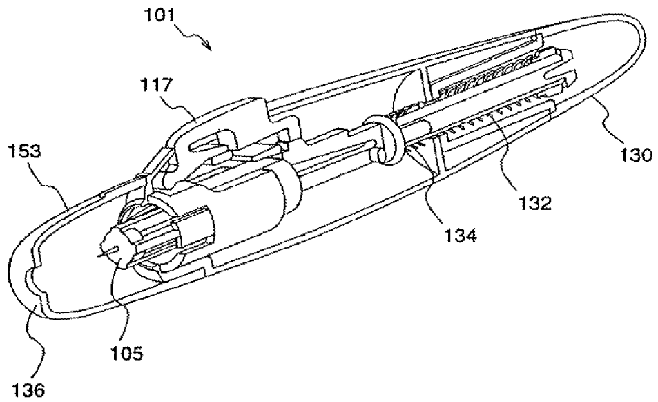
Fig.13 Prior Art
