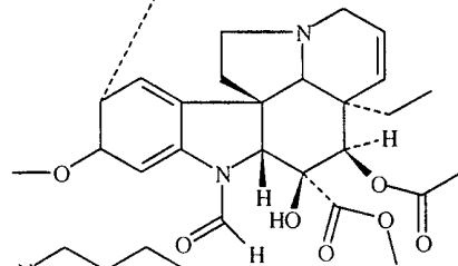
Vincristine
