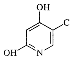
CDHP
