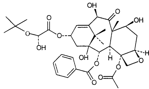
Taxotere
