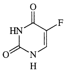
Fluorouracil (5-FU)
