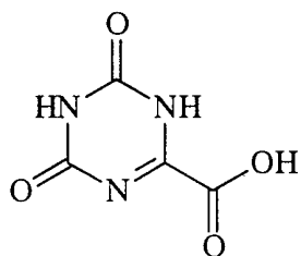
Oxonic Acid
