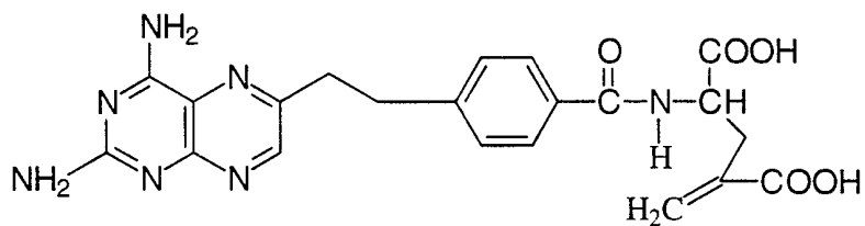
γ-methylene-10-deaza aminopterin (MDAM)
