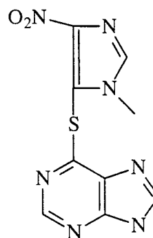
Azathioprine
