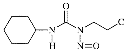
Lomustine (CCNU)
