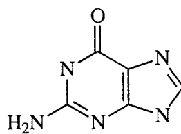
Guanine
