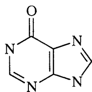
Hypoxanthine
