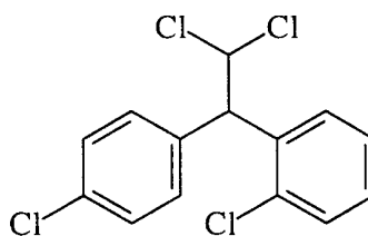
Mitotane
