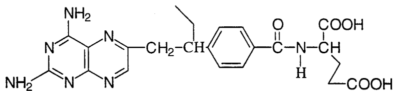
10-ethyl-10-deaza aminopterin (EDAM)
