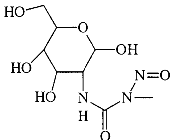
Streptozocin
