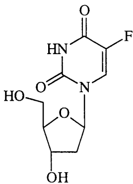
Floxuridine
