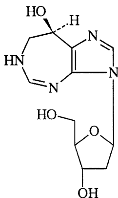
Pentostatin
