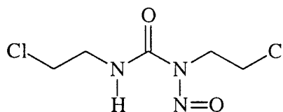
Carmustine (BCNU)
