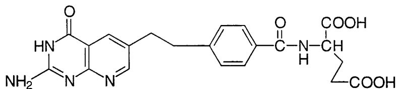
5,10-dideaza tetrahydrofolate
