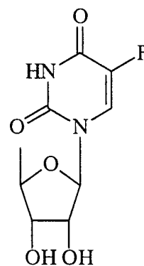
5'-deoxyfluorouridin
