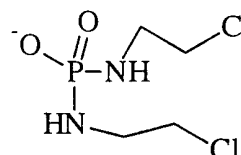
Isophosphoramidate Mustard
