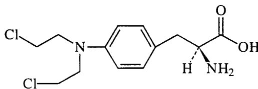
Melphalan
