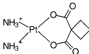
Carboplatin
