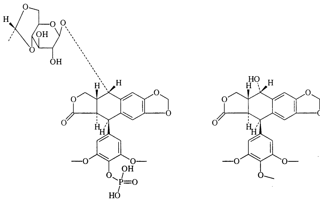
Podophyllotoxin
