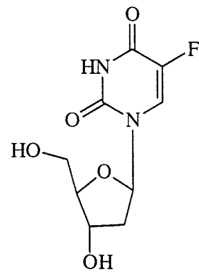
Floxuridine
