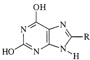
R=H=Xanthine R=OH=Uric Acid
