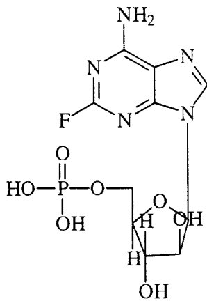
Fludarabine Phosphate
