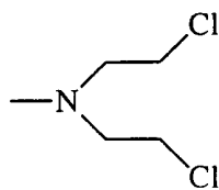
Mechlorethamine
