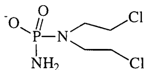
Phosphoramidate Mustard
