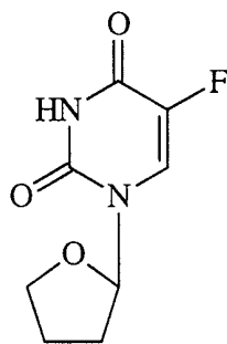
Ftorafur
