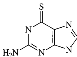
6-Thioguanine
