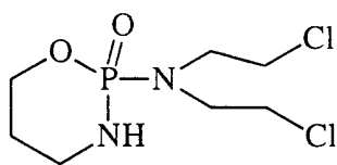
Cyclophosphamide
