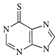
6-Mercaptopurine
