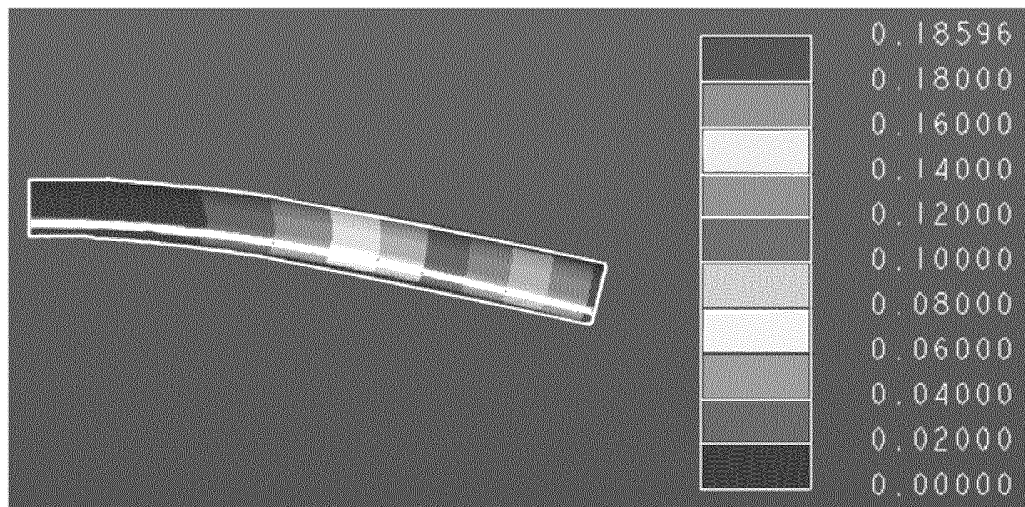
<UP-DOWN AIRFLOW DIRECTION PLATE 27X>
