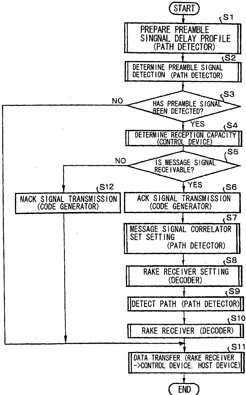
FIG. 7 [PRACH CALLING PROCESSING SEQUENCE]
