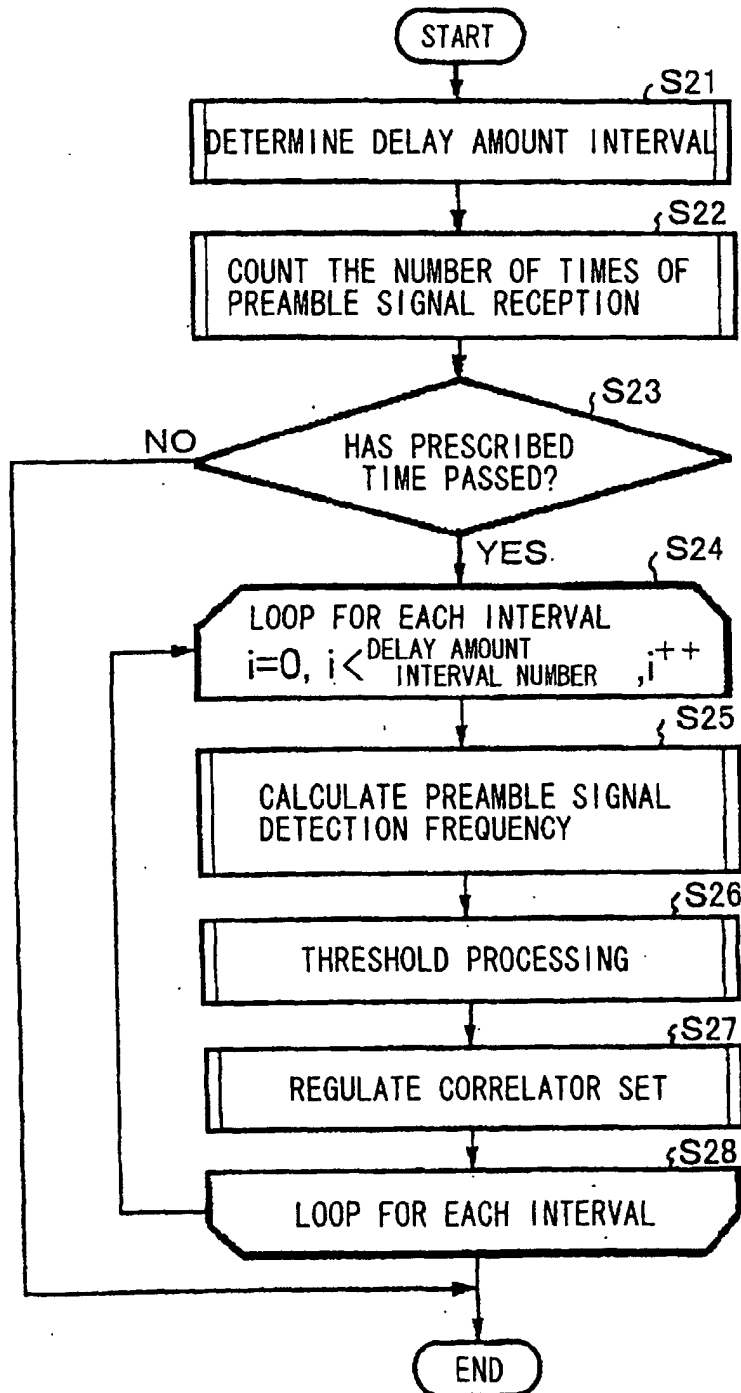
FIG. 8 [PROCESSING SEQUENCE CONCERNING CORRELATOR SET MANAGEMENT]
