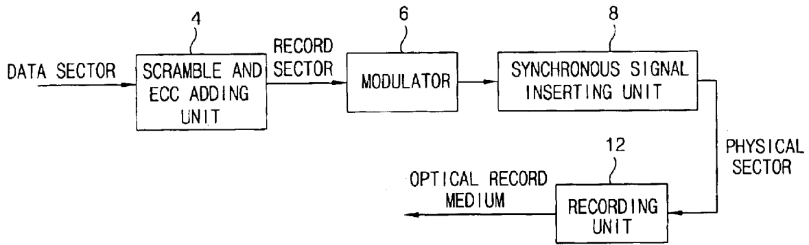
FIG. 4 CONVENTIONAL ART
