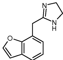
a) 2-Benzofuran-7-ylmethyl-4,5-dihydro-1-imidazole
