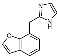
a) 2-Benzofuran-7-ylmethyl-4,5-dihydro-1-imidazole
