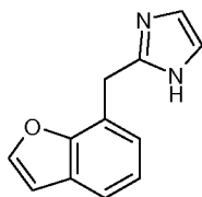
b) 2-Benzofuran-7-ylmethyl-1H-imidazole
