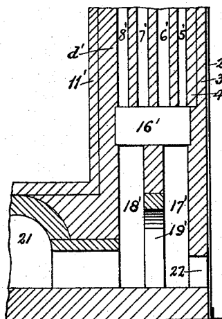
Section III-III
