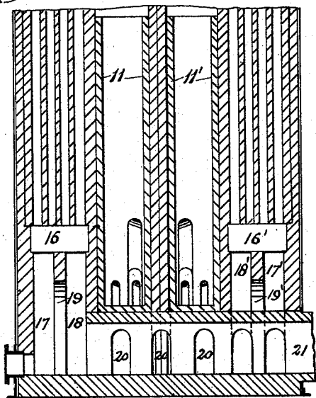
Section I-I
