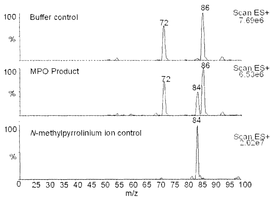
Figure 10. Positive-ion electrospray ionization mass spectrometry (ESI-MS) analysis.
