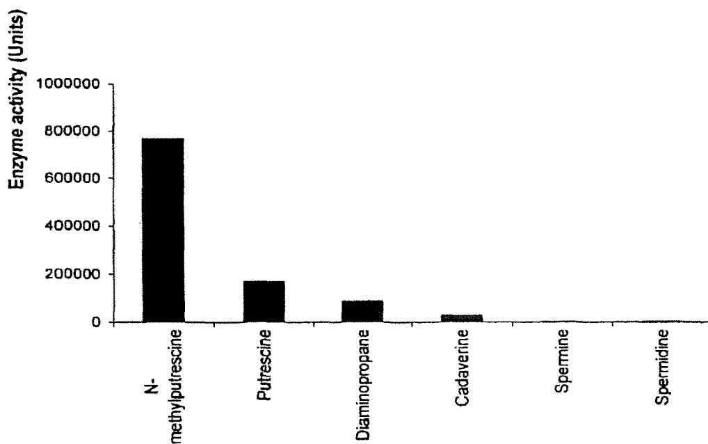
Figure 9. Substrate preference of recombinant MPO enzyme.
