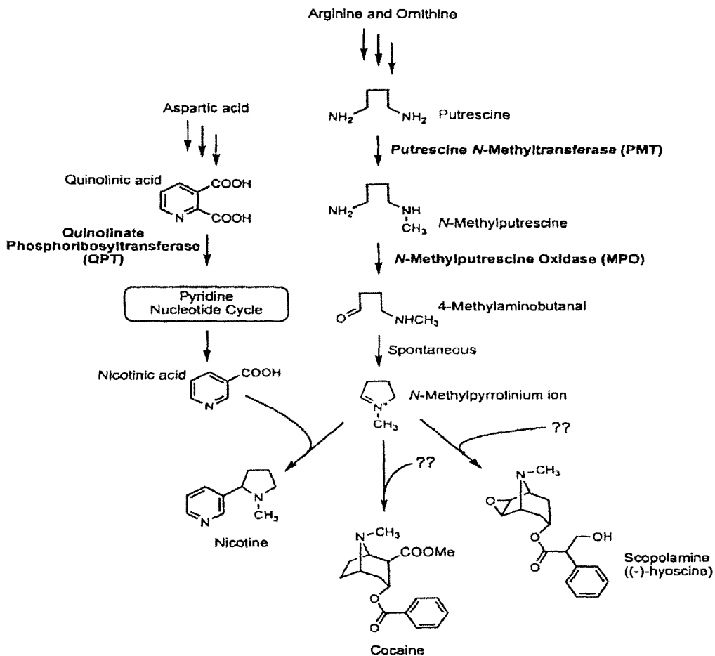
Figure 1. Proposed biosynthetic pathways leading to nicotine and tropane alkaloids (e.g. cocaine and scopolamine) showing the key role of N -methylputrescine oxidase (MPO).
