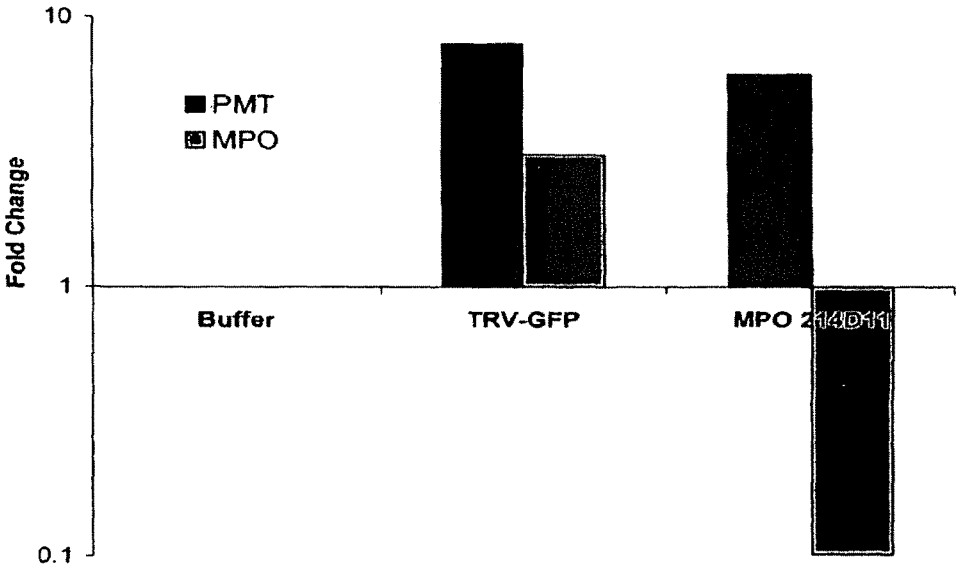
Figure 7. qRT-PCR analysis of MPO and PMT expression in buffer and TRV-GFP control plants, and in MPO-silenced plants infected with TRV-MPO (214D11).
